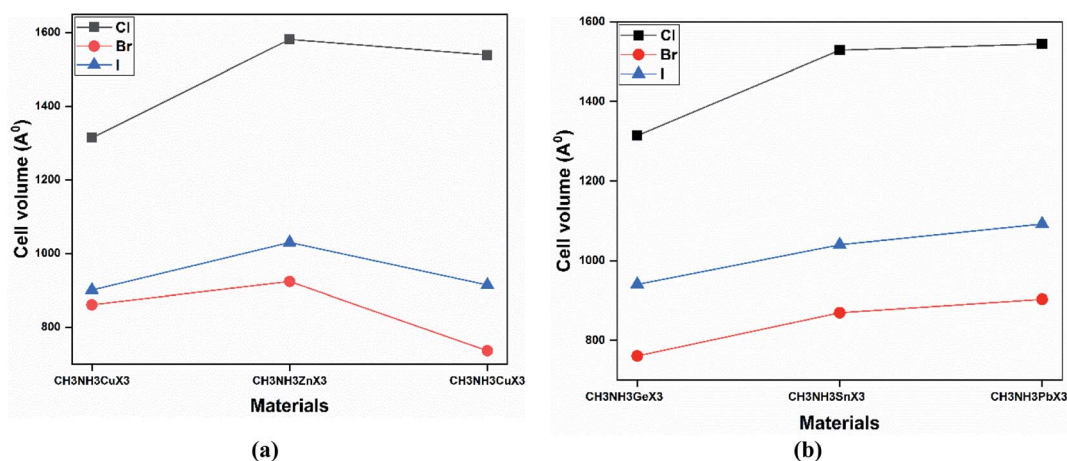
Fig. 3 A comparison of the cell volume (in Å 3 ) values upon varying the metal and halide at the GGA-PBE level of theory for (a) same-period and (b) same-group perovskite compounds.
