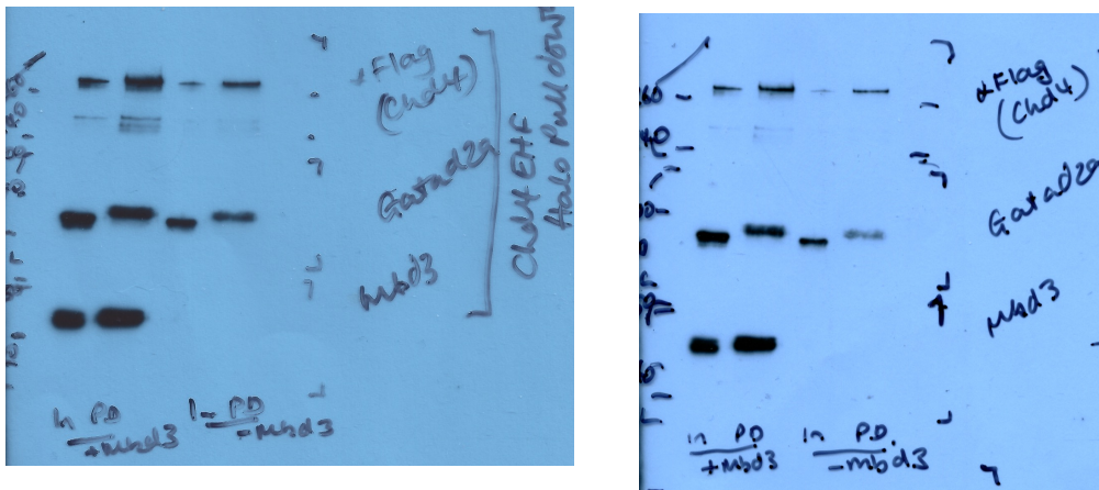
CHD4 Pull down / Probed \alpha Flag/Gatad2a/Mbd3 (Duplicate experiment, two exposures)
