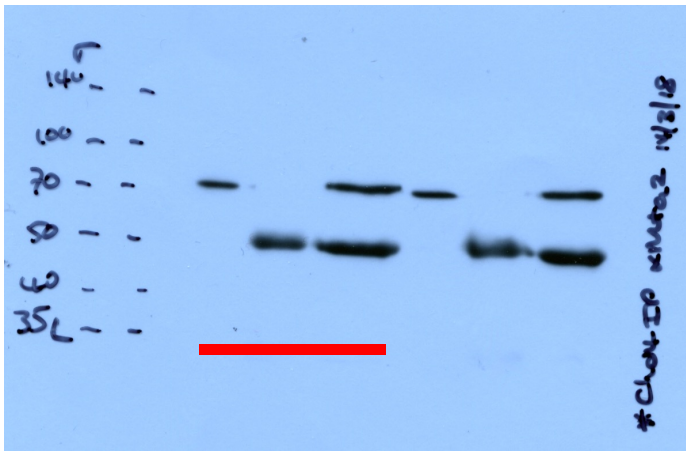
\alpha CHD4 IP/ Probed \alpha MTA2
