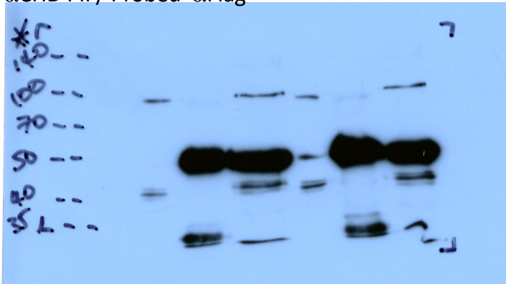
\alpha CHD4 IP/ Probed \alpha Flag
