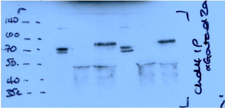
\alpha CHD4 IP/ Probed \alpha GATAD2A
