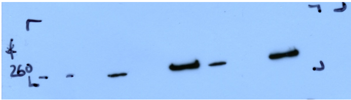
\alpha CHD4 IP/ Probed \alpha CHD4
