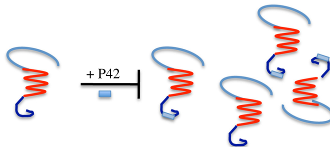
Fig. 2 Model of action of P42. A- In pathogenic conditions, cleavage of mutant polyQhtt is increased, leading to short N-terminal fragments mostly lacking P42. N17 domains self interact, bringing together polyQhtt proteins (nucleation step). Oligomers will further form parallel \beta sheets, thereby enhancing the aggregation process [64]. B- Our model is that exogenous addition of P42 allows a protective effect of polyQhtt-induced defects by directly interacting with the N17 domain of the N-terminal part of polyQhtt, therefore preventing nucleation, and consequently oligomerisation and aggregation processes.
