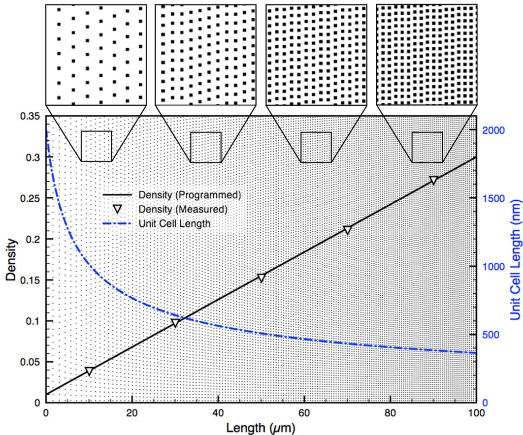
Figure 2. Programmed and measured density for an ordered linear DNG. A 100 \times 100 \mu m^2 linear DNG comprised of 0.04 \mu m^2 nanodots and spanning from 0.01 to 0.30 density. The measured density (left axis) precisely matches the programmed density ( R^2 = 0.9998 ). The unit cell dimensions (right axis) change with the inverse square root of the density. Top insets show various spacing of nanodots at positions along the DNG. doi:10.1371/journal.pone.0106541.g002
