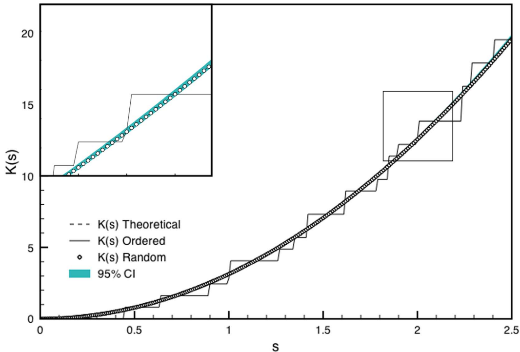
Figure 4. Ripley's K analysis for randomness and spatial homogeneity of a sample box produced with the ordered and random DNG algorithms. K(s) for ordered and random gradients for a 10 \times 400 \mu\text{m}^2 box at 0.20 density are shown. A 95% confidence interval was calculated as 1.96 times the standard deviation of K(s) from 10 simulations of randomly distributed points at 0.20 density. The inset shows a magnified portion of the graph indicated by the box. doi:10.1371/journal.pone.0106541.g004
