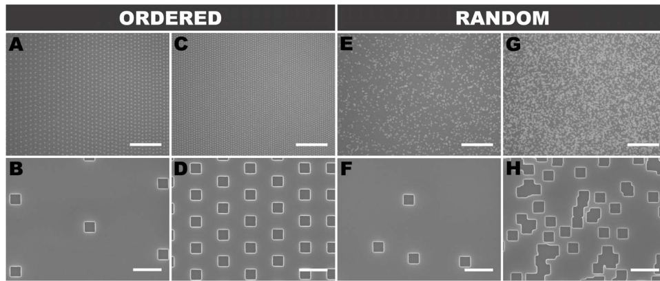
Figure 8. Nanodot distribution in ordered and random DNGs. SEMs of ordered (A–D) and random (E–H) exponential gradients at low (A,B,E,F) and high (C,D,G,H) densities. (H) highlights the random overlap between nanodots that is compensated for by the random DNG algorithm. Scale bars are 10 \mu\text{m} (top row) and 500 nm (bottom row). doi:10.1371/journal.pone.0106541.g008
