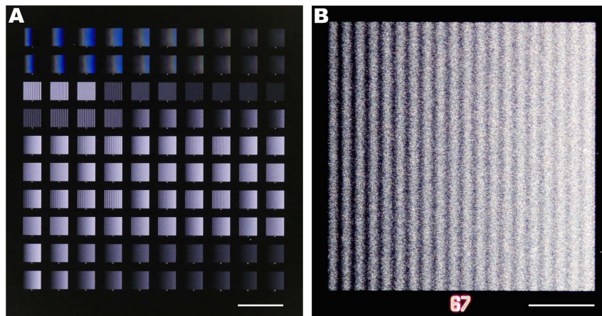
Figure 7. Optical images of the 100-gradient-array. The 100 DNGs were patterned into a Si wafer using e-beam lithography. (A) Image of all gradients; scale bar is 1 mm. (B) Dark-field image of DNG 67 which is a random sinusoid with exponentially increasing average density; scale bar is 100 µm. doi:10.1371/journal.pone.0106541.g007
