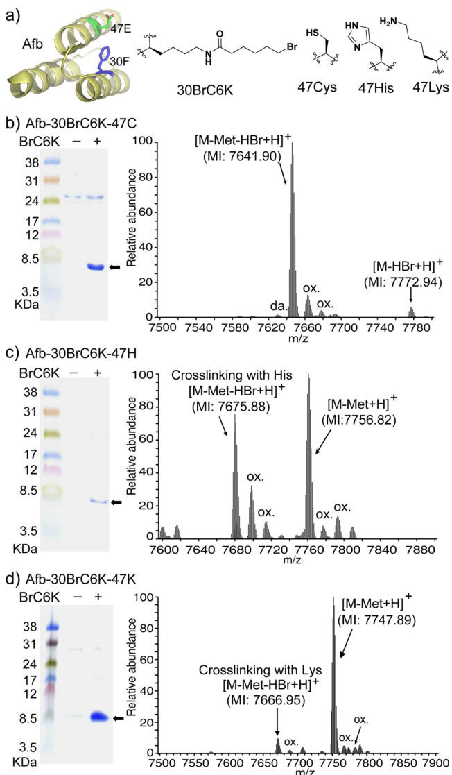
Figure 2. BrC6K is able to target His and Lys in addition to Cys in intramolecular PEPC. (a) Crystal structure of the Afb (PDB ID: 1LLP1) showing the two proximal sites F30 and E47 used for introducing BrC6K and Cys/His/Lys, respectively. (b–d) SDS-PAGE (left panels) and high resolution ESI-FTMS (right panels) analyses of affibody mutant proteins Afb-30Uaa-47C (b), Afb-30Uaa-47H (c), and Afb-30Uaa-47K (d). The cross-linking reaction of the Uaa with Cys/His/Lys all result in the loss of HBr. Peaks were observed with monoisotopic masses corresponding to Afb containing the covalent bond formed between the Uaa and the respective target Cys, His, and Lys in each sample. For BrC6K-Cys cross-linked product [M – HBr + H], expected 7772.97 Da, measured 7772.94 Da; [M – Met – HBr + H], expected 7641.93 Da, measured 7641.90 Da. For BrC6K-His cross-linked product [M – Met – HBr + H], expected 7675.98 Da, measured 7675.88 Da. For BrC6K-Lys cross-linked product [M – Met – HBr + H], expected 7667.01 Da, measured 7666.95 Da. da., deamidation; ox., oxidation.
