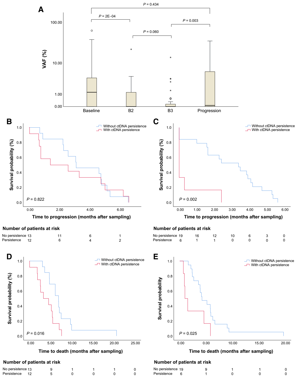
Figure 3. Dynamic changes in ctDNA during treatment. A , Boxplot of ctDNA VAF at baseline, 1 (B2) and 2 months (B3) after initiation of chemotherapy, and at the time of progression ( n = 32 ). B , Progression-free survival in patients without ctDNA persistence versus patients with ctDNA persistence 1 month after initiation of chemotherapy and (C) 2 months after initiation of chemotherapy. D , Overall survival in patients without ctDNA persistence versus patients with ctDNA persistence 1 month after initiation of chemotherapy and (E) 2 months after initiation of chemotherapy.
