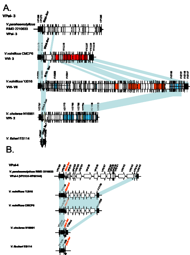
Figure 2 A and B. Schematic representation of V. parahaemolyticus island-3 (VPal-3) and VPal-4, and the homologous insertion site among the 4 sequenced Vibrio species. Block arrows represent annotated ORFs. Black filled in ORFs represent core chromosomal flanking genes. Open and shaded arrows represent genomic island ORFs. Shaded blocks indicate homologous ORFs among the Vibrio species.
