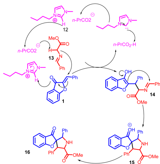
Scheme 5 Proposed mechanism for the synthesis of pyrrolidine and 1-indanone derivatives.
