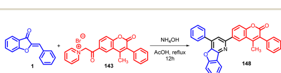
Scheme 47 Synthesis of modified pyridine-substituted coumarins from aurones.
