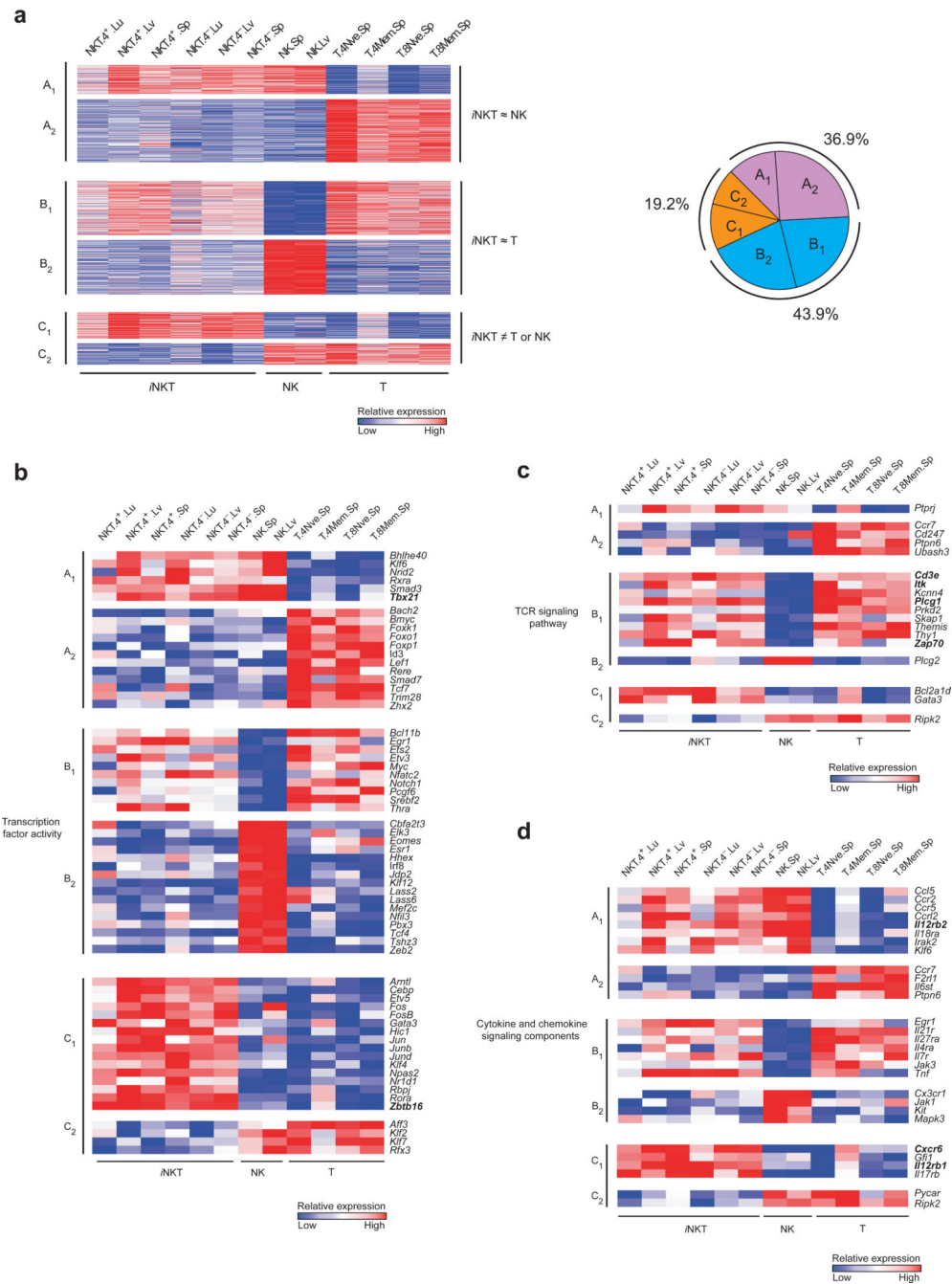
Fig. 4. Characterization of shared and differential gene expression among i NKT, NK, and T cells. One-way ANOVA was performed to compare gene expression in i NKT, NK, and T cell populations. Differentially expressed genes were separated into six categories depending on common patterns in 2 of the 3 subsets. Genes up- (A 1 ) or down- (A 2 ) regulated in NK and i NKT compared to T cells; genes up- (B 1 ) or down- (B 2 ) regulated in i NKT and T compared to NK cells; genes up- (C 1 ) or down- (C 2 ) regulated in i NKT compared to T or NK cells. (a) Left , heatmap of genes expressed differentially in i NKT, NK, and T cells for the indicated
