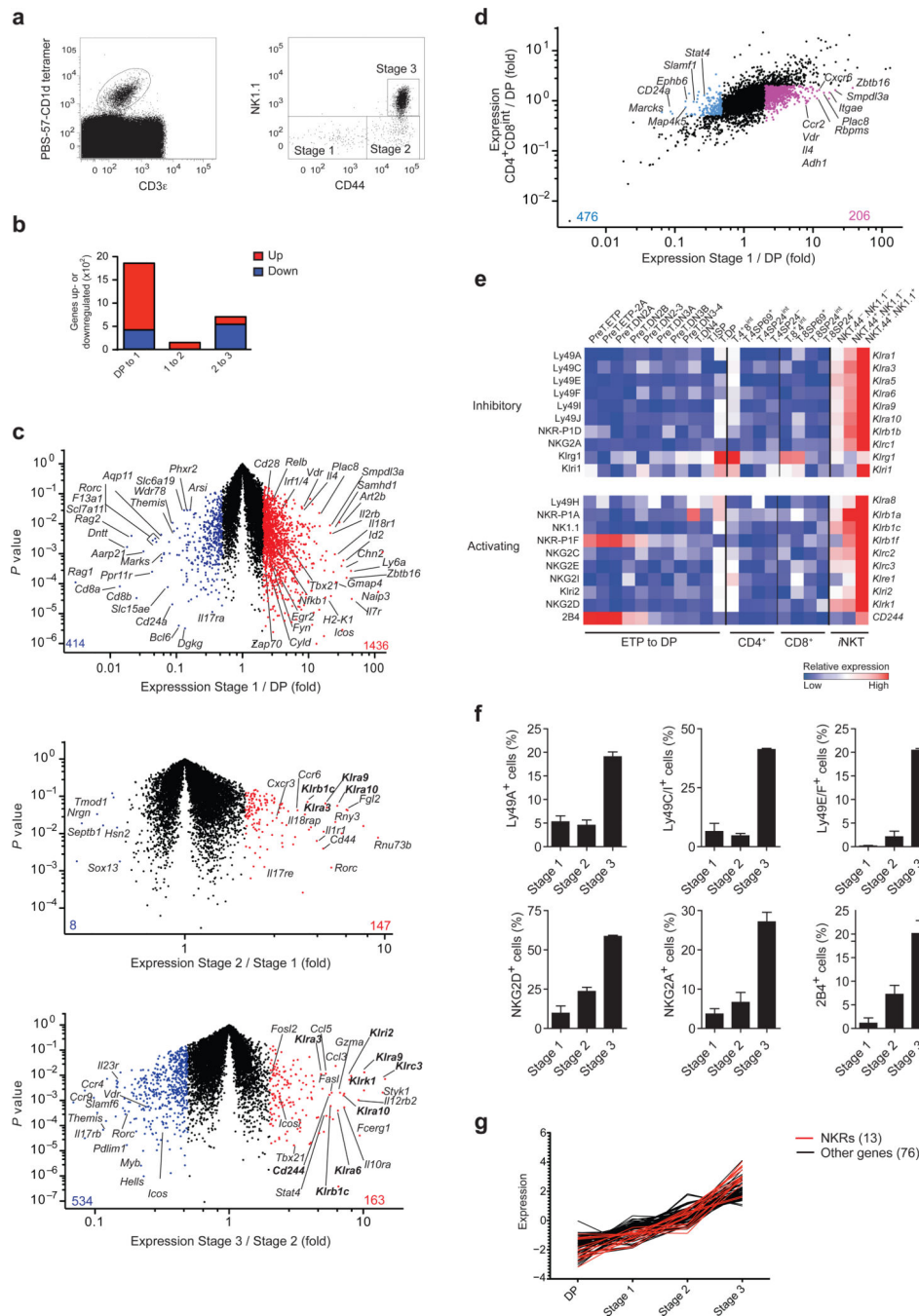
Fig. 1. i NKT cells upregulate NKR at the end of thymic differentiation. (a) Flow cytometric identification of thymic i NKT cells. (b) Number of genes differentially expressed during i NKT cell developmental transitions. (c) Genes differentially expressed between DP thymocytes and stage 1 (top), stage 1 and stage 2 (middle), and stage 2 and stage 3 i NKT cells (bottom). Genes upregulated are highlighted in red or blue, respectively. See Supplementary Tables 1–6 for complete lists. (d) Genes differentially expressed in stage 1 i NKT cells versus DP thymocytes. Colored highlights indicate genes differentially regulated
