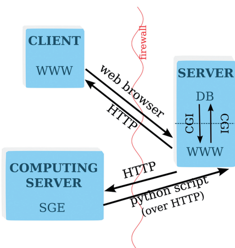
Figure 2. Interaction between the computing cluster(s), the front-end server and the user.
