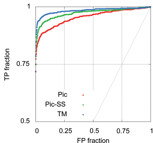
Figure 3. ROC curves for SCOP Family assignment obtained by three methods: sequence profile alignment (Pic), alignment with secondary structure profiles (Pic-SS) and structure alignment (TM). Area under ROC curve: 0.955, 0.957 and 0.984, respectively.
