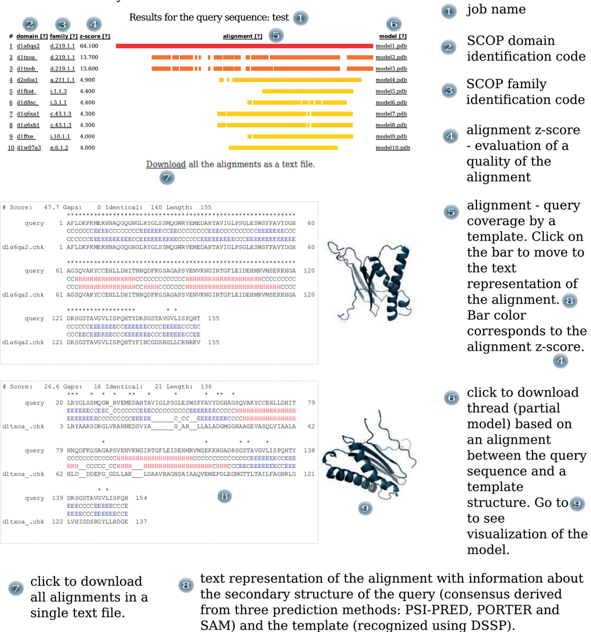
Figure 1. Sample Bioshell Threader result page describes functionalities of the server.
