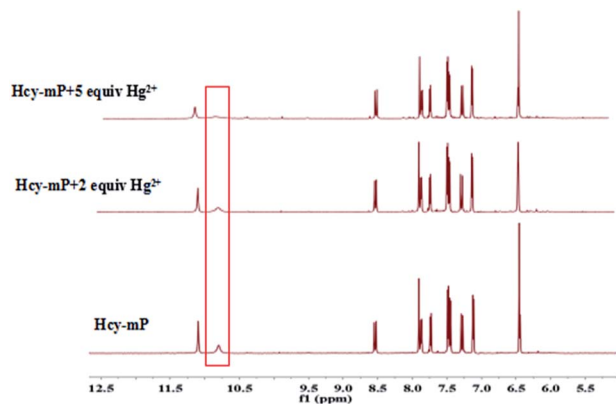
Fig. 9 The ^1\text{H} NMR for Hcy-mP and Hcy-mP + \text{Hg}^{2+} (2, 5 equiv.) in DMSO.
