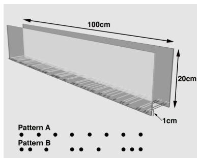
Fig 1. The skilled ladder rung walking test apparatus in the frontolateral view, with the specific measurements of the apparatus indicated. Two different rung patterns were used in the present study: Pattern A, regular rung arrangement, Pattern B, irregular rung arrangement. The irregular rung arrangement varied between consecutive trials.
