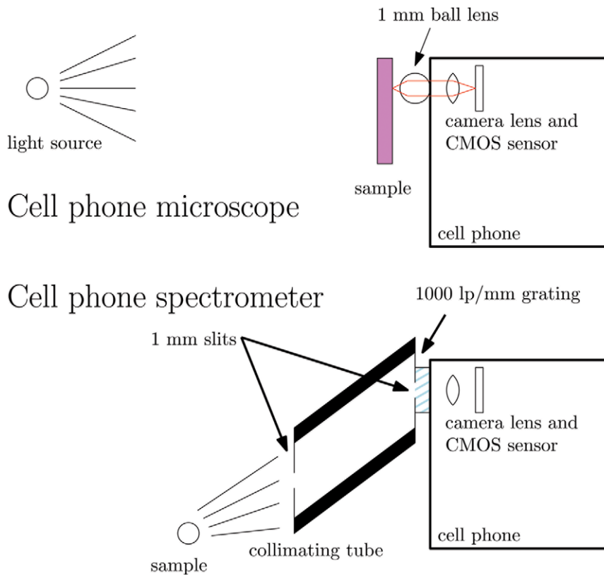
Figure 1. System diagrams. Top panel shows the cell phone microscope achieved by adding a ball lens to the cell phone camera system. Lower panel shows the cell phone spectrometer, constructed by adding a grating and collimating tube to the cell phone camera. doi:10.1371/journal.pone.0017150.g001
