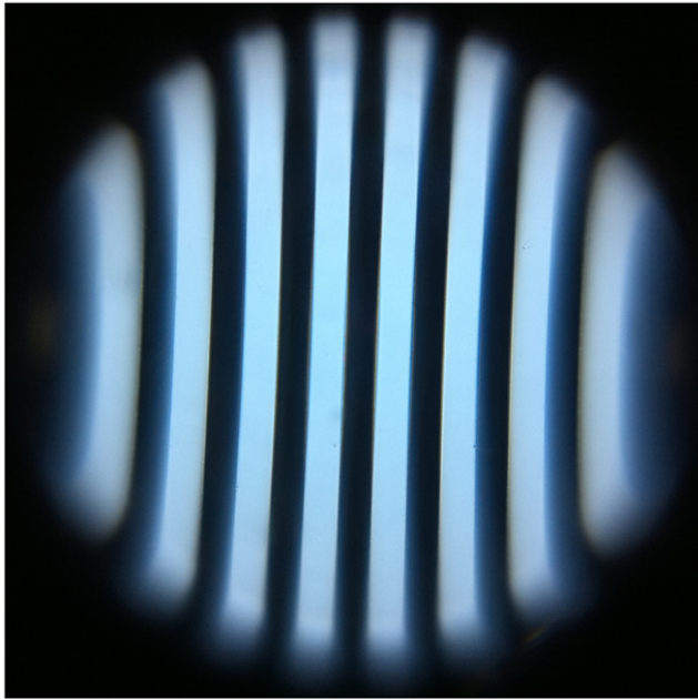
Figure 3. Cropped image of a 20 lp/mm Ronchi ruling using the iPhone 4 microscope. Pincushion distortion and defocus due to field curvature can clearly be seen at the edge of the field-of-view. doi:10.1371/journal.pone.0017150.g003
