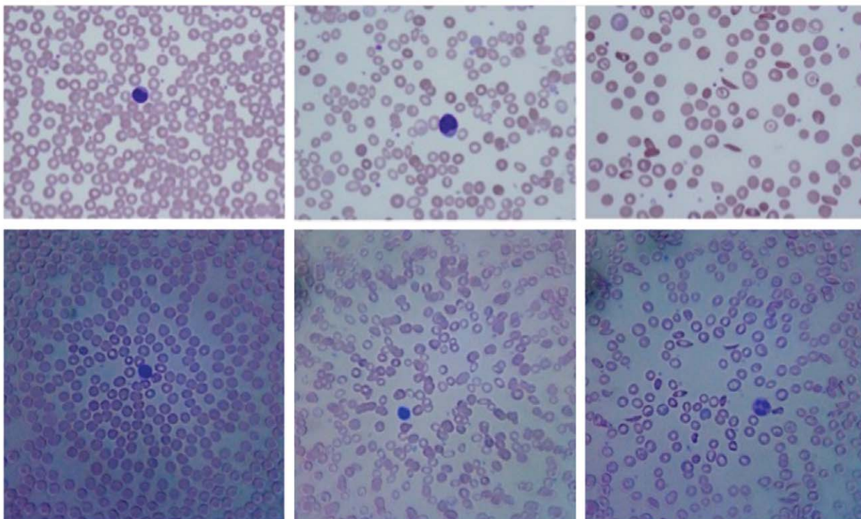
Figure 6. Micrographs of peripheral blood smears. Upper row: images from a traditional microscope. Bottom row: images from a cell phone microscope. Left, blood from a normal patient. Center, blood from a patient suffering from iron deficiency anemia. Right, blood from a patient suffering from sickle cell anemia.
