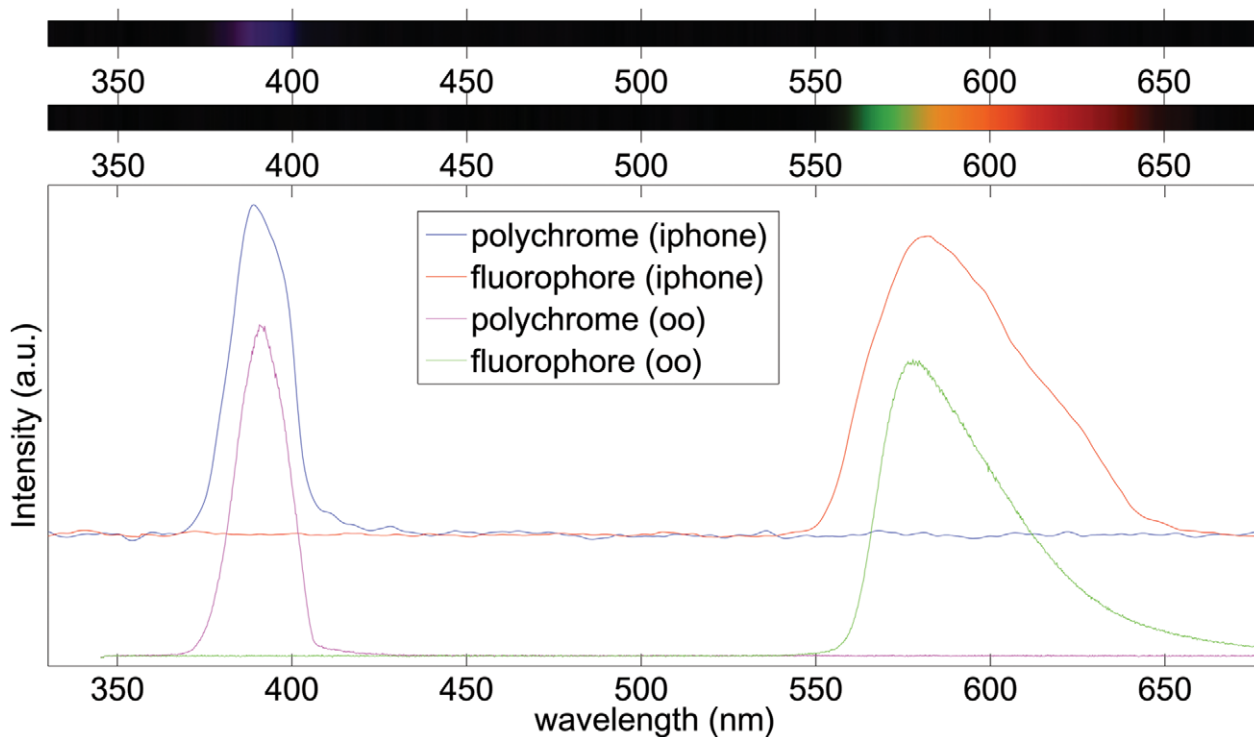
Figure 10. Fluorescence spectrum of rhodamine 6G. Upper panel, image of spectrum of Polychrome V light source. Middle panel, image of rhodamine 6G spectrum. Lower panel, a comparison of the excitation and emission spectra of the Polychrome V and rhodamine 6G taken with the cell phone spectrometer and validated with the commercial Ocean Optics spectrometer (oo). doi:10.1371/journal.pone.0017150.g010
