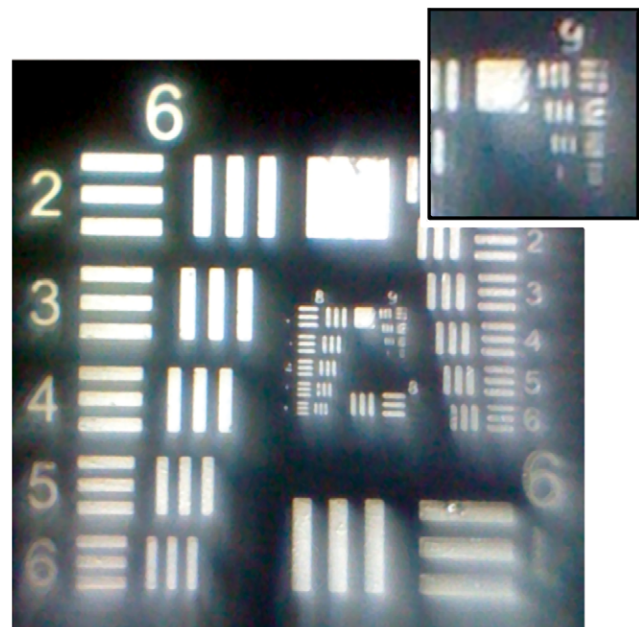
Figure 2. USAF resolution target. Image of resolution target taken with the iPhone 2G microscope, showing the ability to clearly resolve group 9 element 2, with slight distortions at the edge of the field. doi:10.1371/journal.pone.0017150.g002
