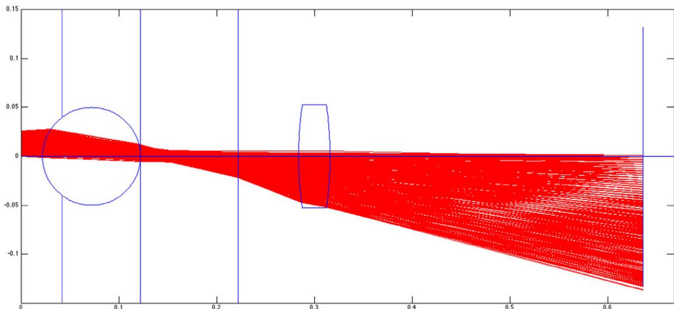
Figure 13. Raytracing simulation result. Trace of 10^7 rays through a system composed of an 800 micron aperture, 1 mm ball lens, plastic biconvex lens, and CMOS sensor. Dimensions of plastic lens and sensor correspond to those in the iPhone 2G. doi:10.1371/journal.pone.0017150.g013
