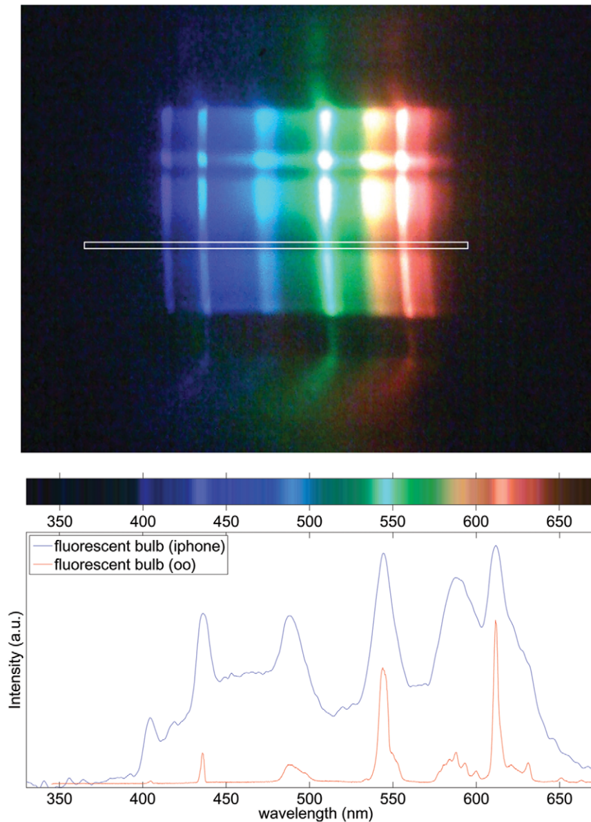
Figure 8. Image and spectrum of fluorescent bulb. Top panel, cropped image recorded by the cell phone spectrometer pointed at a standard fluorescent light fixture. White box indicates area used to determine spectrum in lower panel. Lower panel (top), an image of the spectrum corresponding to area in the white box in the top panel. Lower panel (bottom), a comparison of the spectra of the same fluorescent light fixture taken with both the cell phone spectrometer (blue) and Ocean Optics (oo) spectrometer (red). doi:10.1371/journal.pone.0017150.g008
