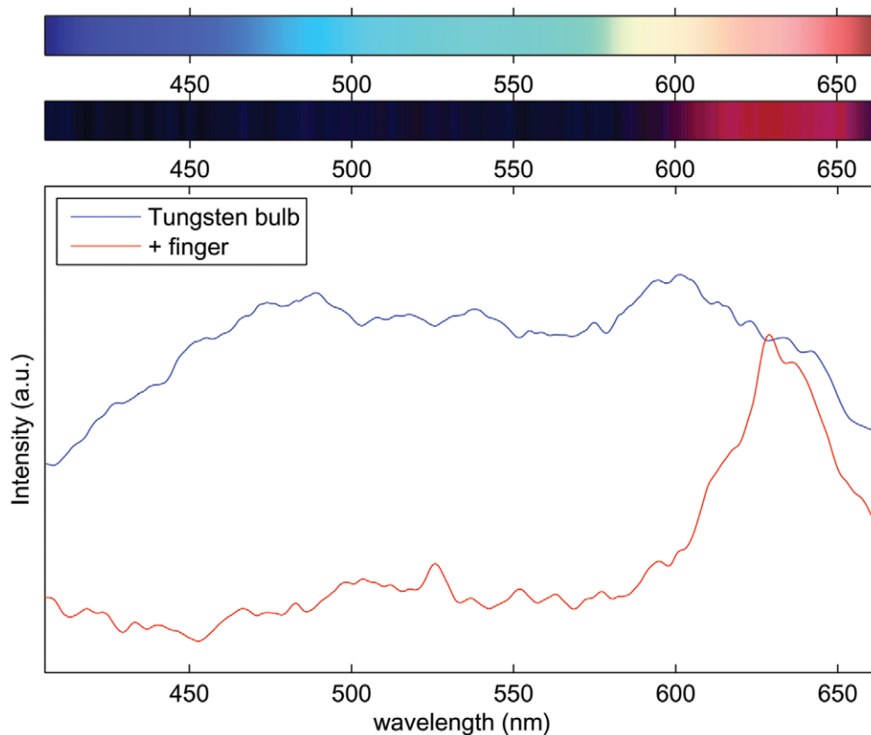
Figure 9. Transmission spectrum of a human finger. Upper panel, image of spectrum corresponding to a tungsten bulb. Middle panel, image of a spectrum corresponding to a tungsten bulb with a finger placed over the slit of the spectrometer. Lower panel, spectra of both the tungsten bulb and the transmission spectrum of the finger. doi:10.1371/journal.pone.0017150.g009
