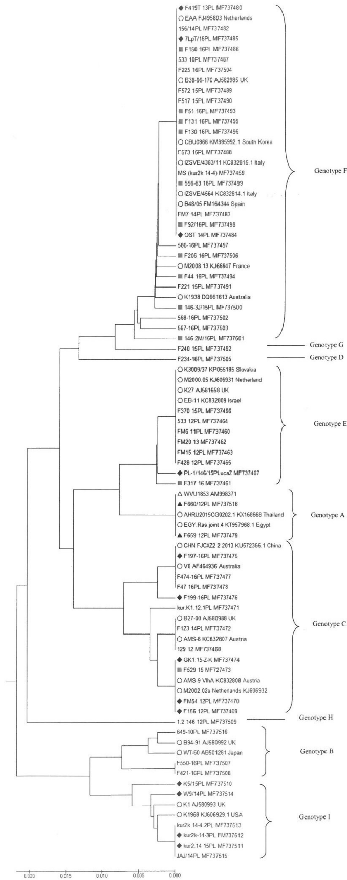
Fig. 2. Phylogenetic tree derived from unweighted pair group method with arithmetic means. It includes 58 Polish MS vlhA sequences corresponding to M. synoviae reference strain WVU1853 and sequences from other countries. The empty triangle is the reference sequence, and empty circles represent sequences from other countries. Filled squares are sequences from chickens showing reproductive disorders, filled diamonds are those from chickens showing respiratory signs, and filled triangles are those from chickens with swollen joints
