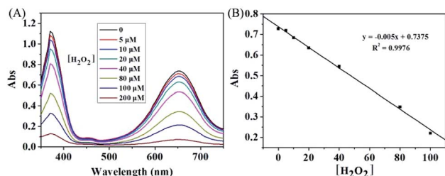
Fig. 3 (A) The absorption spectra of the \text{KMnO}_4 -TMB system for analyzing different concentrations of \text{H}_2\text{O}_2 . (B) Calibration curve of \text{H}_2\text{O}_2 in the range from 5 to 100 \mu\text{M} . The data shown here represent the average of three independent experiments.
