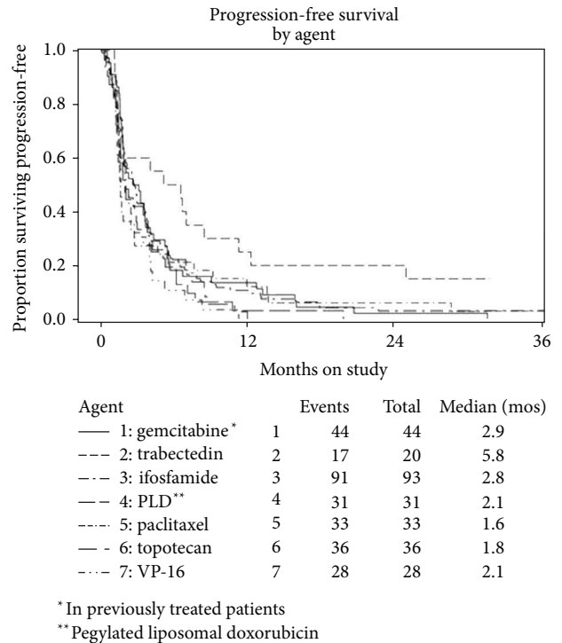
FIGURE 1: Kaplan–Meier plots demonstrating progression-free survival (PFS) for the 20 patients in the study population (GOG 87M) compared to other single agent studies in the GOG protocol 87 series studying cytotoxic agents. Reprinted from [49], with permission from Elsevier.
