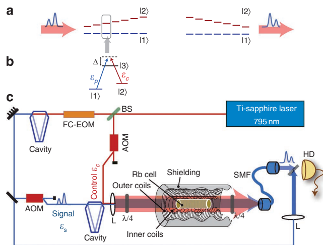
Figure 1 | Schematic view of the experiment. (a) Schematic view of the frequency gradient generated for an ensemble of two-level atoms. By switching the sign of the gradient from positive (left) to negative (right) a photon-echo is emitted in the forward direction. (b) Schematic view of \Lambda -atom structure, which at large detuning is equivalent to a two-level atom based on the two ground states. (c) Experimental setup showing the control (red) and signal (blue) beams with 6.8 GHz frequency difference, collimated at radii of 6 and 3 mm, respectively, and of identical circular polarization when they go through the cell. Heterodyne measurement is performed after the memory on the signal field. AOM, acousto-optic modulator; BS, beam splitter; FC-EOM, fibre-coupled electro-optic modulator; HD, heterodyne detection; SMF: single-mode fibre; \epsilon_s and \epsilon_c , signal and control field amplitudes, respectively.
