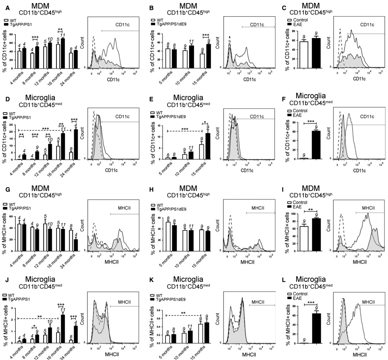
Fig. 2 Analyses of microglia and MDM activation states in two AD models and EAE mice. CD11c (A–F) and MHCII (G–L) expression on CD11b + CD45 high MDM populations (A–C and G–I) and CD11b + CD45 med microglia (D–F and J–L) from WT littermate controls, TgAPP/PS1 mice (A, D, G, J), TgAPP/PS1dE9 mice (B, E, H, K), and EAE mice. Gates shown in the FACS histograms (right panel) illustrate CD11c (A–F) and MHCII (G–L) expression in CD11b + CD45 high cells and CD11b + CD45 med cells from WT mice (black histogram) and 16-month-old TgAPP/PS1 mice (A, D, G, J), 15-month-old TgAPP/PS1dE9 mice (B, E, H, K), and EAE mice (C, F, I, L) (black tinted histogram). Isotype antibodies were used as negative controls (dotted histogram). The number of mice is indicated above each histogram bar. Data are expressed as means ± SEM. * P < 0.05, ** P < 0.01, *** P < 0.001 statistical significance.
