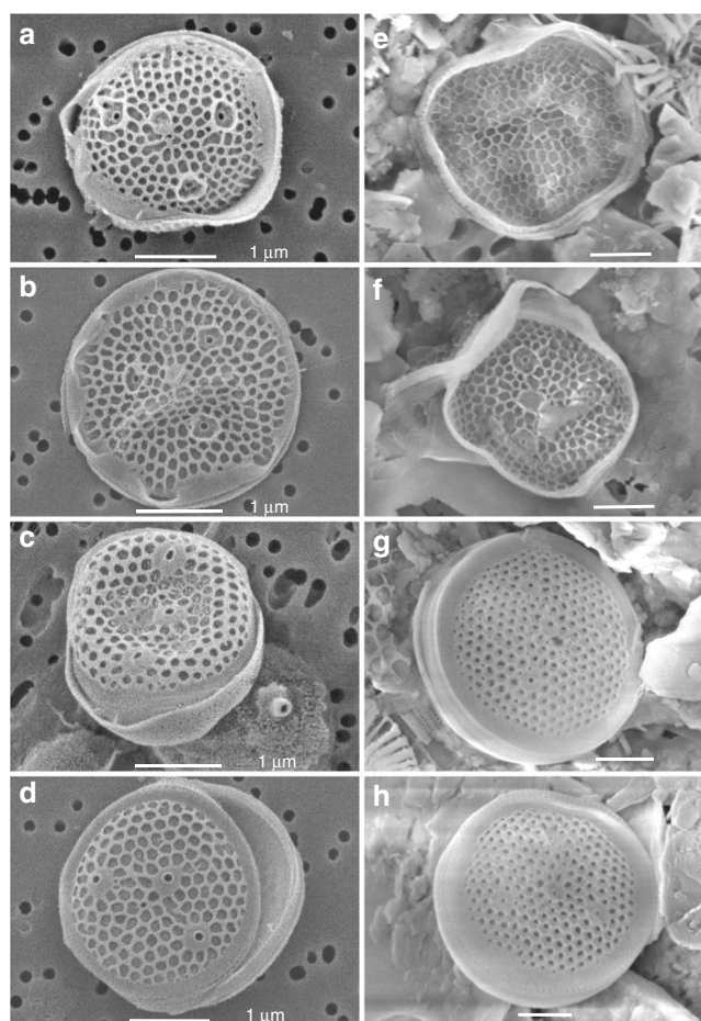
Fig. 5 Minidiscus comicus and Minidiscus trioculatus in surface water and sediment trap samples during spring 2013. (a, b) M. comicus , (c, d) M. trioculatus observed in scanning electron microscopy (SEM) at station 99, located at 42°N, 5°E on 24 th April 2013 at the surface. (e, f) M. comicus , (g, h) M. trioculatus observed in SEM in three deep sediment traps samples (2400 m) at 42°N, 4.5°E covering 30 th March to 22 nd May 2013. All scale bars are 1 \mu\text{m}
