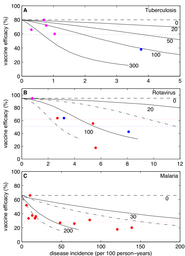
Fig. 1. Vaccine efficacy on disease incidence gradients. (a) Tuberculosis [1]. (b) Rotavirus [2–4]. (c) Malaria [10]. Solid curves are generated with the formula 1 - r_v/r_c , where r_c and r_v represent the incidence of infection in the control and vaccine groups, over 1 year, and the labels indicate the variance of the risk distribution, q(x) , in the absence of vaccination. Dash-dotted lines are the same measures calculated over longer follow-up (2 years in the case of rotavirus, 4 years in the case of malaria). Data points come from settings where a trial has been conducted to estimate vaccine efficacy (Tables S1, S2, and S3), and dotted lines represent average estimates by continent (America (magenta), Asia (blue), Africa (red)) taken from the originally published trial analyses.
