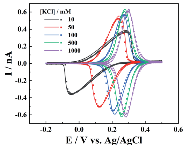
Fig. 5 Experimental (solid lines) and simulated (points) i - V curves for different concentrations of KCl ( c_1 ). The \text{K}_4\text{Fe}(\text{CN})_6 concentration is 1 mM. c_1 , mM: 10 , 50 , 100 , 500 , and 1000 . a = 50 nm, d = 1100a , \tan \theta = 0.19 , \nu = 0.1 V \text{s}^{-1} and E_0 is 0.12 , 0.18 , 0.24 , 0.265 , and 0.29 V.
