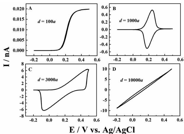
Fig. 3 Simulated i - V responses from a CNP at different solution depths in 1 mM \text{K}_4\text{Fe}(\text{CN})_6 + 0.1 M KCl. From panels (A) to (D), the solution depth is 100a , 1000a , 3000a , and 10\,000a . a = 50 nm, \tan \theta = 0.2 , \nu = 0.1 V \text{s}^{-1} and E^0 = 0.2 V.
