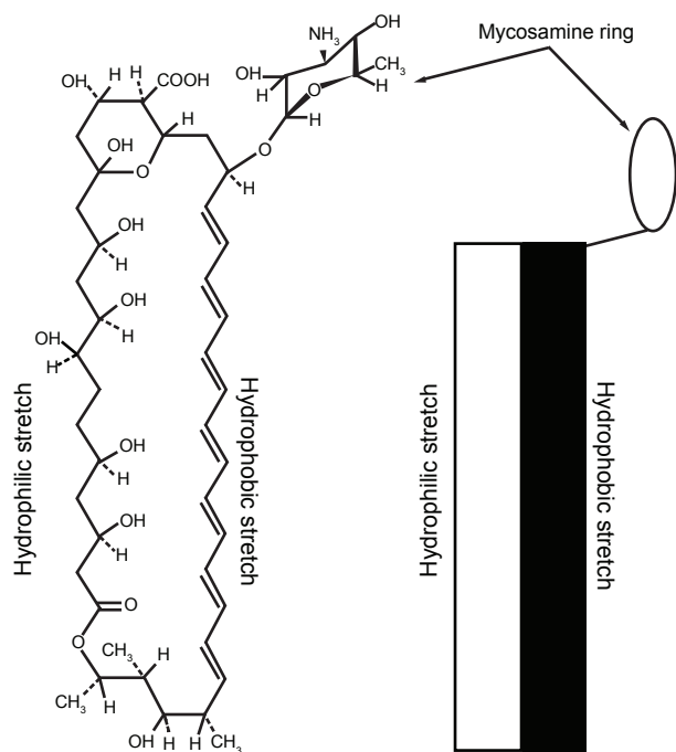
Figure 1 Structure of Amphotericin B.
