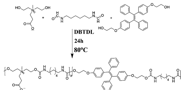
Scheme 2 Detailed synthetic route of the TPE-CB PUs.
