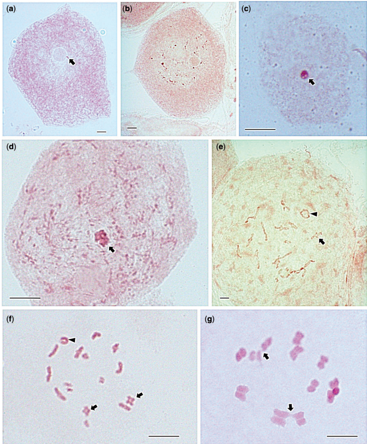
Fig. 2. Cells of the seminiferous tubules of R. c. crassifemur (a), G. f. flavus (b, e), B. micantum (c), M. brasiliensis (d), B. anurum (f), and M. uruguayensis (g) stained with lacto-acetic orcein. (a) Prophase I with a small heteropycnotic corpuscle near the nucleolus (arrow); (b) prophase I with several small heteropycnotic corpuscles; (c) prophase I with heteropycnotic corpuscle (arrow); (d) prophase I with a large corpuscle heteropycnotic, rounded with no defined morphology (arrow); (e, f) diplotene/diakinesis with interstitial chiasmata that give the chromosome a cross-shaped morphology (arrow) or double terminal chiasmata that give the chromosomes a rounded morphology (arrowhead); (g) diplotene/diakinesis with telomeric associations between the autosomes (arrow). Bars: 10 \mu m.
