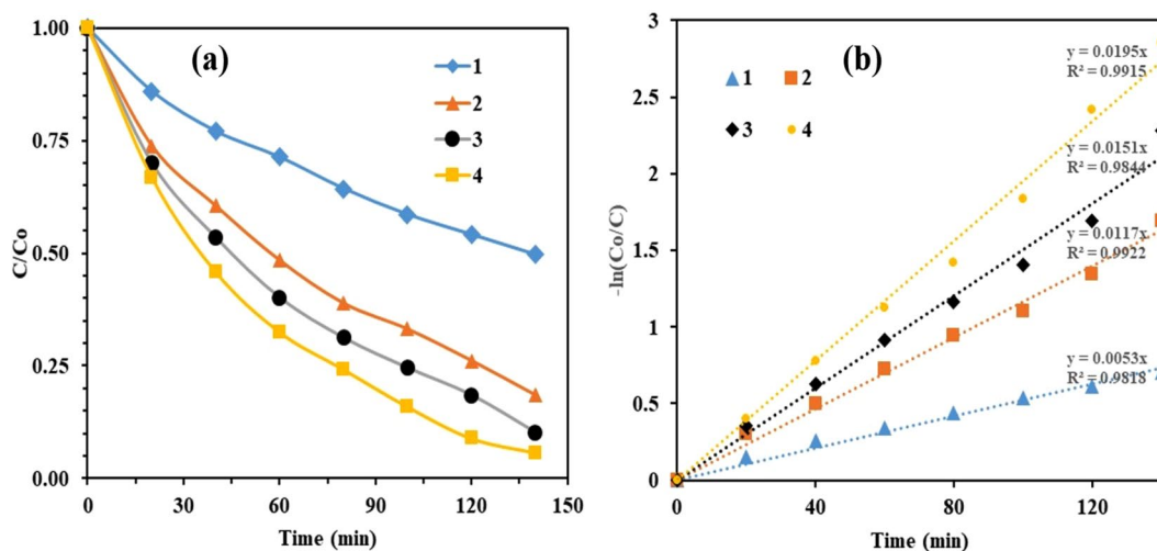
Figure 14. (a) Degradation and (b) reaction kinetics of BPA: pH = 3, catalyst concentration = 140 mg l -1 , and [BPA] 0 = 30 mg l -1 (1) TiO 2 , (2) TCo 0.5 N 1.5 , (3) TCo 1.0 N 1.0 and (4) TCo 1.5 N 0.5 .
