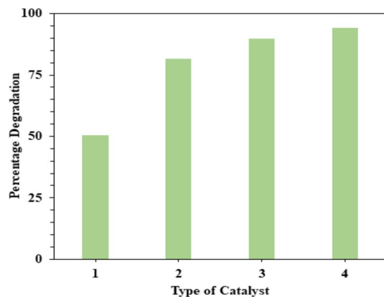
Figure 13. Effect of dopant content for the degradation of BPA: pH = 3, catalyst concentration = 140 mg l -1 , and [BPA] 0 = 30 mg l -1 (1) TiO 2 , (2) TCo 0.5 N 1.5 , (3) TCo 1.0 N 1.0 and (4) TCo 1.5 N 0.5 .
