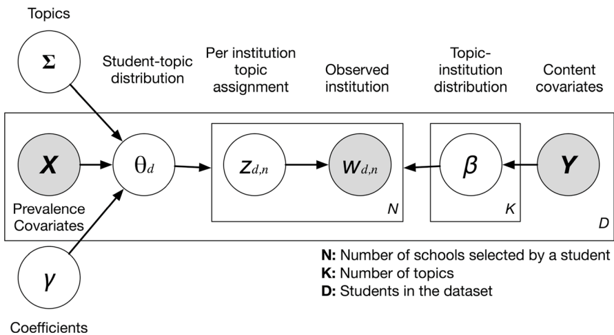
Fig. 1 Graphical illustration of the structural topic model. Grey nodes indicate observable variables. We use the term ‘topic’ to refer to the latent-preference groups estimated by the model
