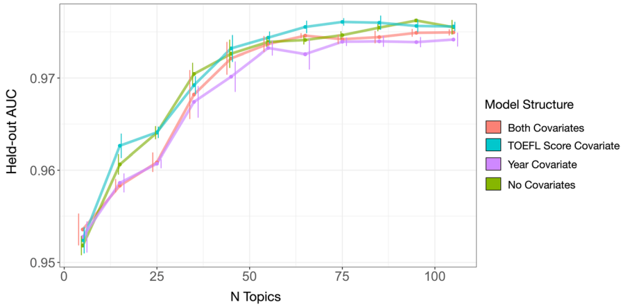
Fig. 2 Mean AUC for our held-out participants for 5-105 topic models. Error bars reflect 1 standard deviation in the means across 5 hold-out validation folds. Colors reflect the 4 different covariate structures we tested
