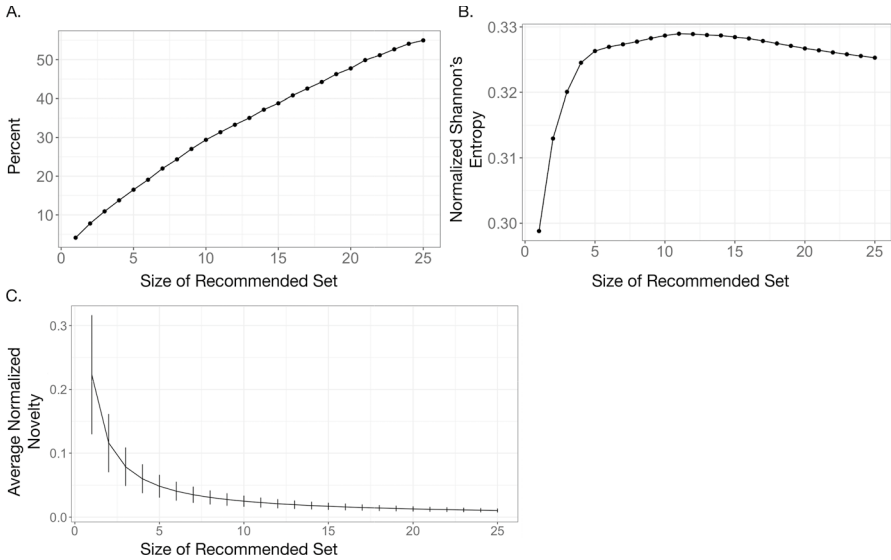
Fig. 6 Item-based beyond-accuracy measures A) Coverage: percent of institutions in entire dataset recommended across top 1-25 recommendations. B) Spread: Entropy of recommendations across top 1-25 recommendations. C) Novelty: The average normalized novelty of institutions within the first 1-25 recommended institutions
