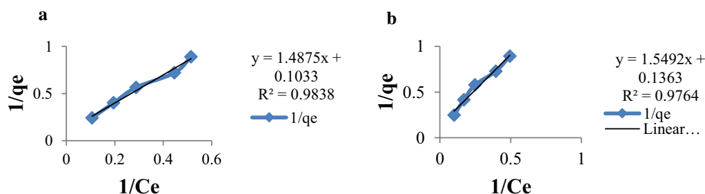
Fig. 9 Langmuir adsorption isotherms for: a chromium by MSSP and b chromium by BPP
