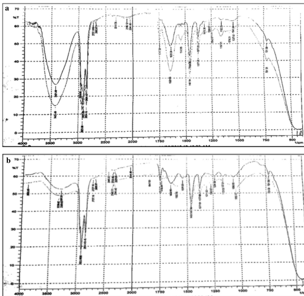
Fig. 3 FT-IR spectra of a BPP and MSSP before adsorption, b BPP and MSSP after adsorption
