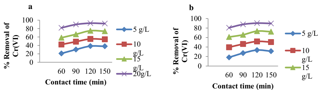
Fig. 4 Effect of contact time on % removal of: A/Cr(VI) by MSSP and B/Cr(VI) by BPP (concentration 30 mg/L, contact time 60, 90, 120 and 150 min, adsorbent dose 5, 10, 15 and 20 g/L solution, agitation speed 150 rpm and pH=2 for MSSP, pH=4 for BPP)
