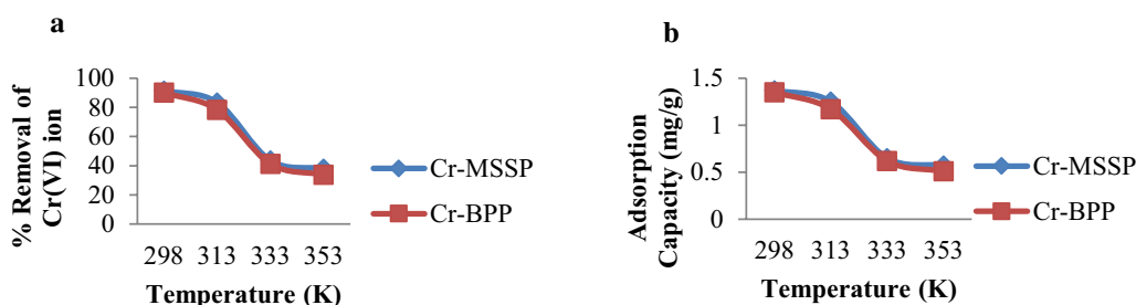
Fig. 8 Effect of temperature on: a % removal of Cr(VI) and b adsorption capacity of MSSP [concentration 30 mg/L, dose 20 g/L, contact time 120 min. and pH 2 for Cr(VI) by MSSP and pH 4 for Cr(VI) by BPP]
