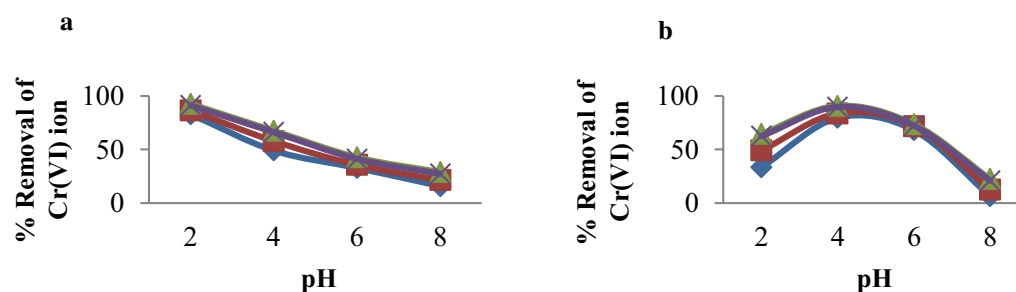
Fig. 5 Effect of solution pH on % removal of: a Cr(VI) by MSSP and b Cr(VI) by BPP (concentration 30 mg/L, pH, 2, 4, 6 and 8 and contact time 60, 90, 120 and 150 min, agitation speed 150 rpm)
