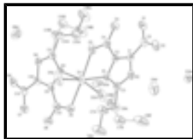
Fig. 1. Molecular structure of the title compound. Displacement ellipsoids are shown at the 30% probability level. Open bonds show minor disordered sites. H atoms have been omitted for clarity.
