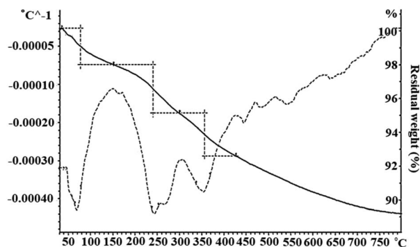
Fig. 3 The TGA/DTGA thermogram of \text{Fe}_3\text{O}_4@SiO_2-[MnL(OAc)] .
