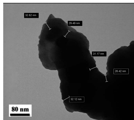
Fig. 5 TEM image of \text{Fe}_3\text{O}_4@SiO_2-[MnL(OAc)] .
