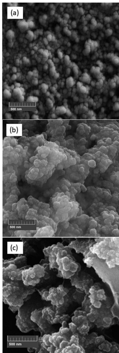
Fig. 4 SEM images of (a) \text{Fe}_3\text{O}_4 , (b) \text{Fe}_3\text{O}_4@SiO_2 , and (c) \text{Fe}_3\text{O}_4@SiO_2-[MnL(OAc)] .
