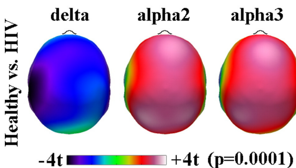
Fig. 9. Topographical maps of statistical values at electrode (sensor) level for frequency bands that presented at baseline most statistical significant differences between Healthy and naïve HIV groups (i.e. delta, alpha 2 and alpha 3).
