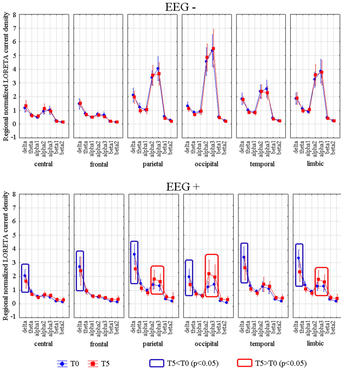
Fig. 5. Top: Mean regional normalized LORETA solutions relative to a statistically non-significant ANOVA interaction ( p > 0.9 ) among the factors Time (T0, T5), Band (delta, theta, alpha 1, alpha 2, alpha 3, beta 1, beta 2), and ROI (central, frontal, parietal, occipital, temporal, limbic) for the sub-group of treatment-naïve HIV subjects with a normal EEG marker (i.e. EEG -). Bottom: Mean regional normalized LORETA solutions relative to a statistically significant ANOVA interaction ( F(30, 3120) = 14.649, p < 0.0001 ) among the factors Time, Band, and ROI for the sub-group of treatment-naïve HIV subjects with a statistically deviant EEG marker (i.e. EEG +).
