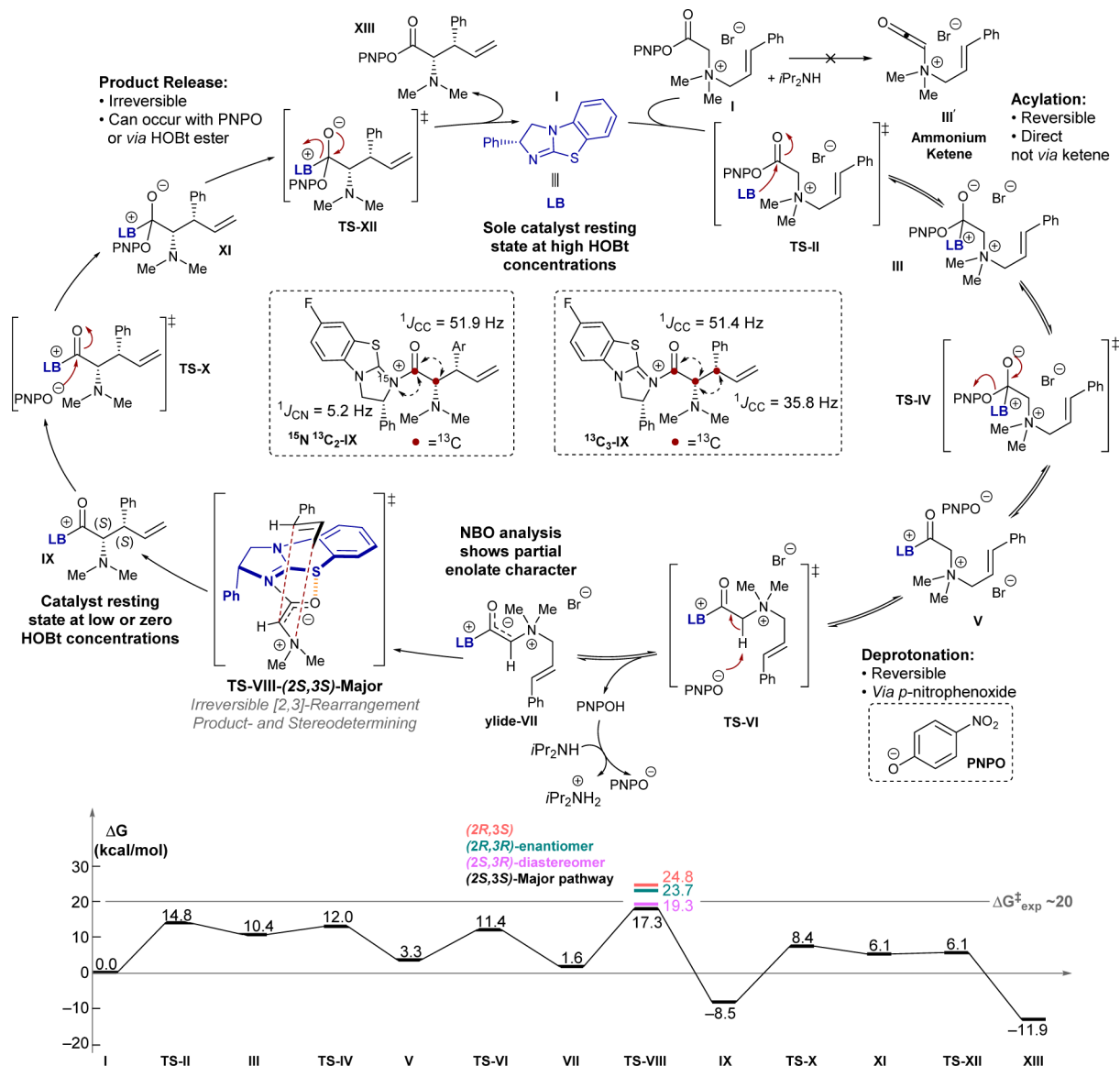
Scheme 9. Proposed Catalytic Cycle and Computed Reaction Coordinate
