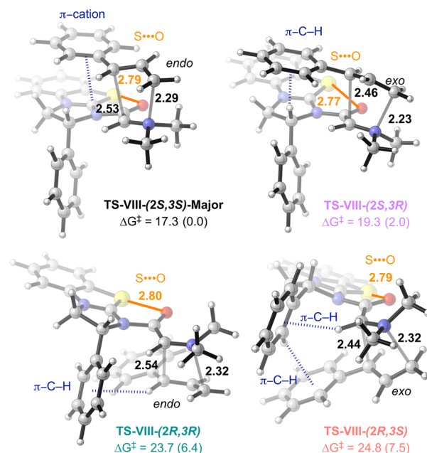
Figure 7. Stereodetermining [2,3]-rearrangement TSs. 34 All energies in kcal·mol -1 , and distances in Å. Shaded gray lines represent forming/breaking bonds. Solid orange lines represent nonbonding S...O interactions. Dashed blue lines represent aromatic interactions.
