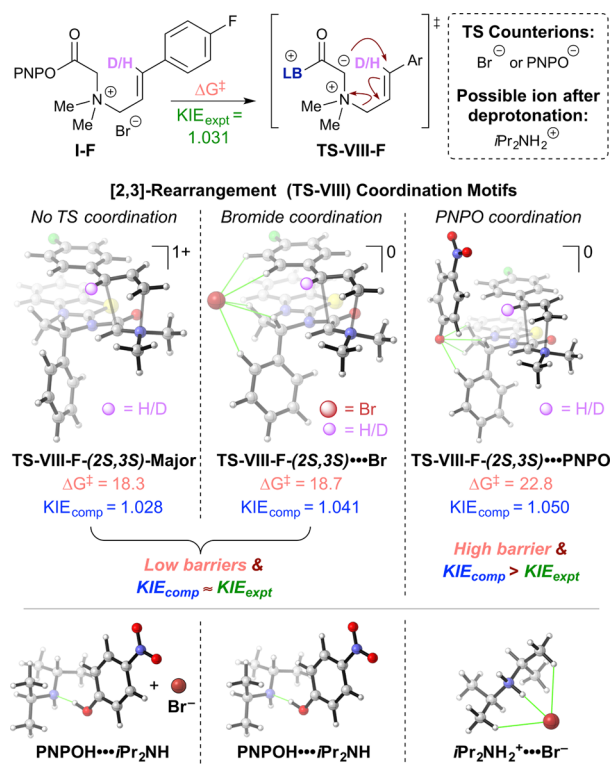
Figure 6. Computed TSs, ions, complexes, and KIEs involving the 4-fluoro substituted substrate I-F. The computed KIE depends on the coordination state of substrate I-F and TS-VIII-F. The violet highlighted atom is the isotopic proton (H/D). 37 All energies in kcal·mol -1 . Shaded gray lines represent forming/breaking bonds. Green lines represent C–H electrostatic interactions and hydrogen bonds.
