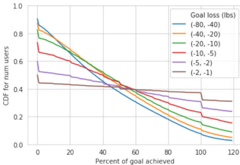
Figure 4: CDF of goal achievement, stratified by goal difficulty. X -axis indicates percent of goal achieved while y -axis indicates the portion of users who have achieved at least that amount of their goal. We find that across the board, goals are unlikely to be achieved. Only 30% of the easiest goals are ever reached, while less than 5% of the most difficult goals are ever reached.
