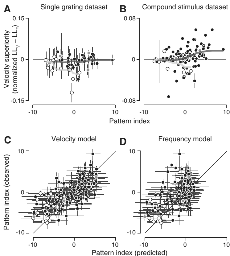
Figure 9. Compound stimuli reveal velocity-separable organization for pattern cells. A, B , Velocity superiority, or the difference of normalized log likelihoods between the velocity and frequency models, per cell as a function of pattern index. V1 cells appear as open circles, MT closed. Example cells featured in Figures 4, 8 are highlighted in gray. Light and dark lines indicate the running mean, with a window of \pm 1/3 of cells in each population. Error bars indicate \pm 1 SD, calculated from model fits to bootstrapped data (note most are smaller than the plotted points). A , On average, for the single grating dataset, neither model better explains the single grating MT data ( A ) for any class of cells ( n = 39 ). The frequency model explains the V1 single grating data better ( n = 13 ). B , Pattern cell responses to the compound stimulus dataset (V1: n = 21 , MT: n = 112 ) are clearly better explained by the velocity model. Error bars indicate \pm 1 SE. C, D , Observed and predicted pattern indices for each cell, derived from the compound stimulus dataset, for the velocity model ( C ) and frequency model ( D ). The velocity model can account for pattern index across all cell types, whereas the frequency model fails to predict the pattern selectivity of neurons classified as pattern-selective based on measured responses. Error bars indicate 95th percentiles, generated from pattern indices calculated by bootstrapping measured and predicted spike trains.
