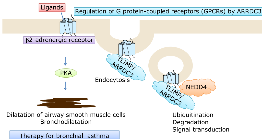
Fig. 4. Regulation of G protein-coupled receptors by TLIMP/ARRDC3. TLIMP/ARRDC3 is reported to interact and co-localize with the \beta 2-adrenergic receptor. (125) The \beta 2-adrenergic receptor is a pharmacologically important G protein-coupled receptor (GPCR) for regulation of dilation of bronchial smooth muscle cells and therapy for bronchial asthma. TLIMP/ARRDC3 may regulate endocytosis, signaling, ubiquitination, and degradation of the \beta 2-adrenergic receptor.
