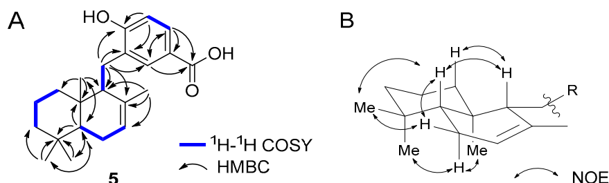
Figure 2. Key COSY, HMBC (A) and NOESY (B) correlations observed in 2D NMR of isozonaic acid ( 5 ).
