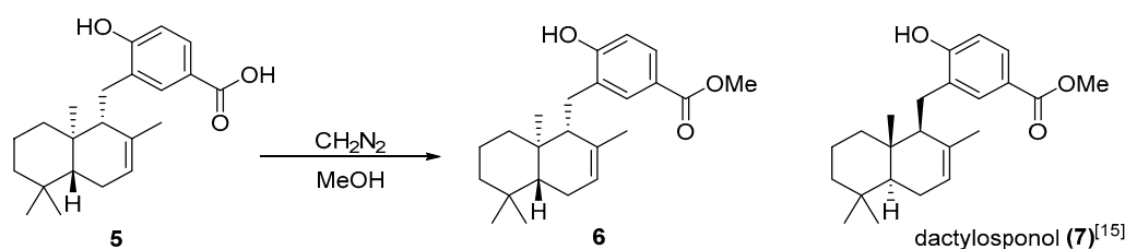
Figure 3. Methyl esterification of isozonaic acid ( 5 ) and structure of dactylosponol ( 7 ).
