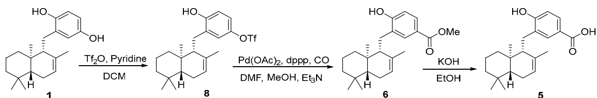
Figure 4. Semisynthesis of isozonaic acid ( 5 ) from isozonarol ( 1 ).
