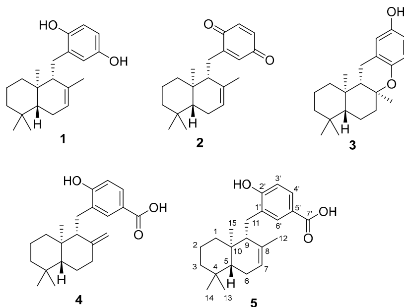
Figure 1. Sesquiterpenoids obtained from D. undulata in this study.
