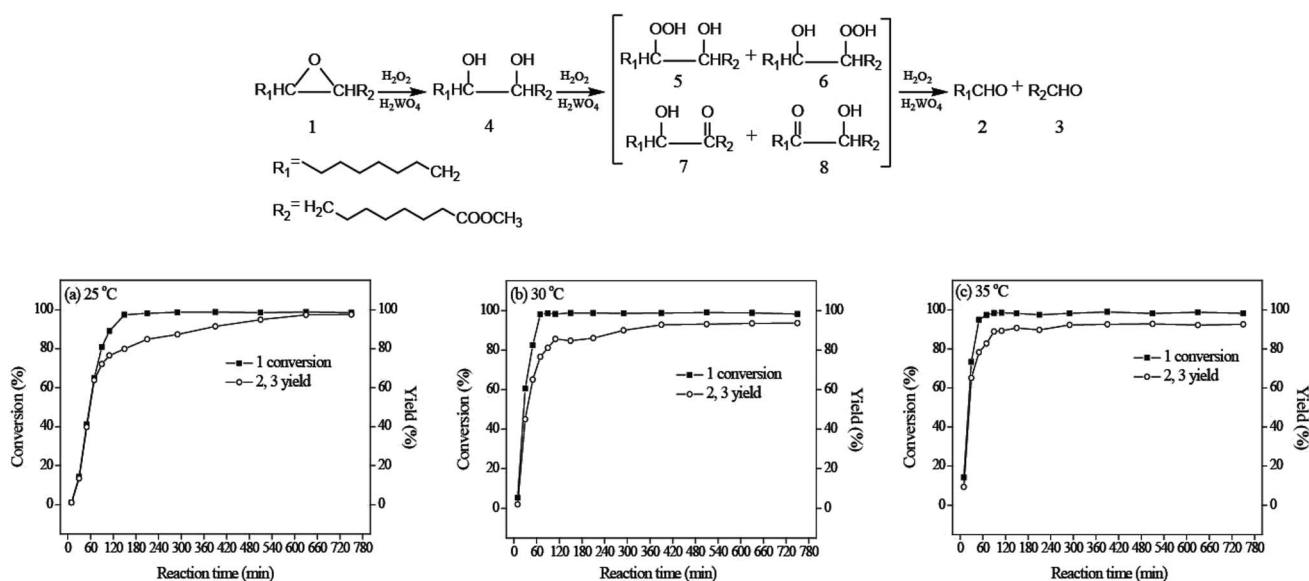
Fig. 1 Effect of reaction time on 1 conversion and aldehyde products ( 2 and 3 ) yields in the temperature range of 25–35 °C (10 mmol epoxide 1 , 12 mmol \text{H}_2\text{O}_2 , 0.17 mmol \text{H}_2\text{WO}_4 , 5 ml t -BuOH).
