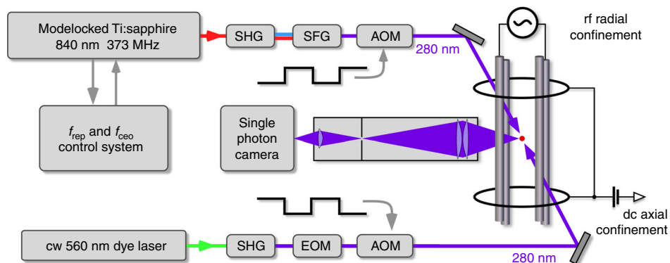
Fig. 1 Experimental setup schematic. A frequency doubled cw dye laser is used for laser cooling trapped Mg ions on the 3s_{1/2}-3p_{3/2} transition. The same transition is interrogated with an individual mode of the UV frequency comb that derives from the third harmonic of a Ti:sapphire mode locked laser and is spatially overlapped with the cw laser. The two lasers are alternately turned on for 2 ms with two acousto optic modulators (AOM). Thanks to its lower power, detuning dependent residual heating/cooling due to the near resonant mode of the comb is largely suppressed (see text). The fluorescence signal is detected by spatially resolved single photon camera during the bright times of the comb i.e. the dark periods of the cooling laser. The ion trap consists of four rf-electrodes, two pairs of ring electrodes for axial confinement and four rod-like dc-electrodes (not shown) for stray field cancellation. SHG second-harmonic generation stage, SFG sum frequency generation stage, EOM electro-optical-modulator
