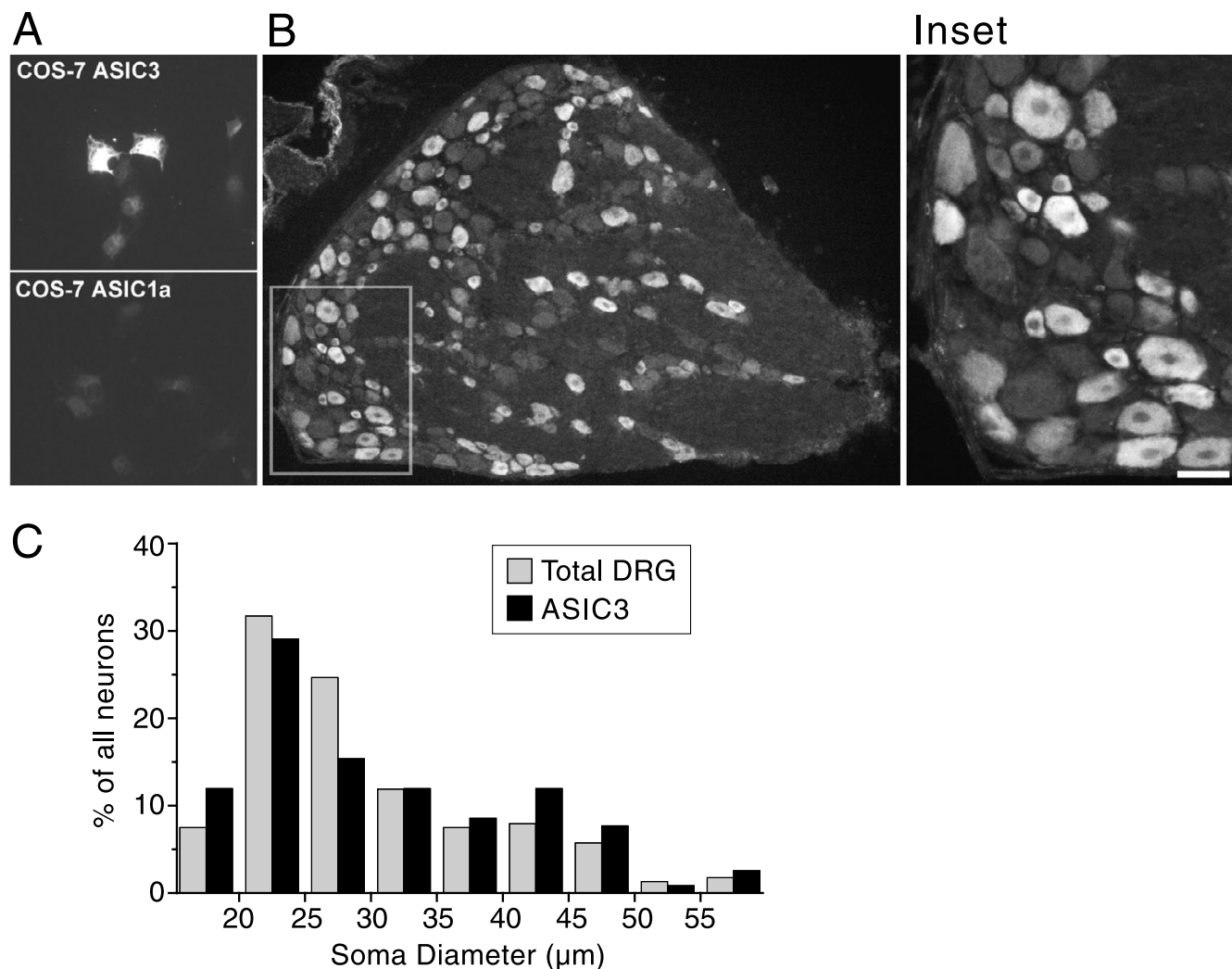
Figure 1 Immunocytochemical localization of ASIC3 in rat sensory neurons. A, ASIC3 antibody labeled COS-7 cells transfected with ASIC3 (top), but not those transfected with ASIC1a (bottom). It also failed to label cells transfected with ASIC1b and ASIC2a (not shown); ASIC2b and ASIC4 were not tested. B, ASIC3 immunoreactivity in a section of L5 DRG. Less than half of neurons are labeled and no non-neurons are labeled. Note the presence of both small and large labeled neurons (inset). Scale bar, 40 μm. C, Size-frequency distribution of ASIC3-positive neurons (black) and of all neurons (grey) from the L5 DRG. ASIC3+ cells are present in all size bins. 3345 neurons (12–15 sections from 3 rats) were counted, of which 1359 (40%) were ASIC3-positive.
