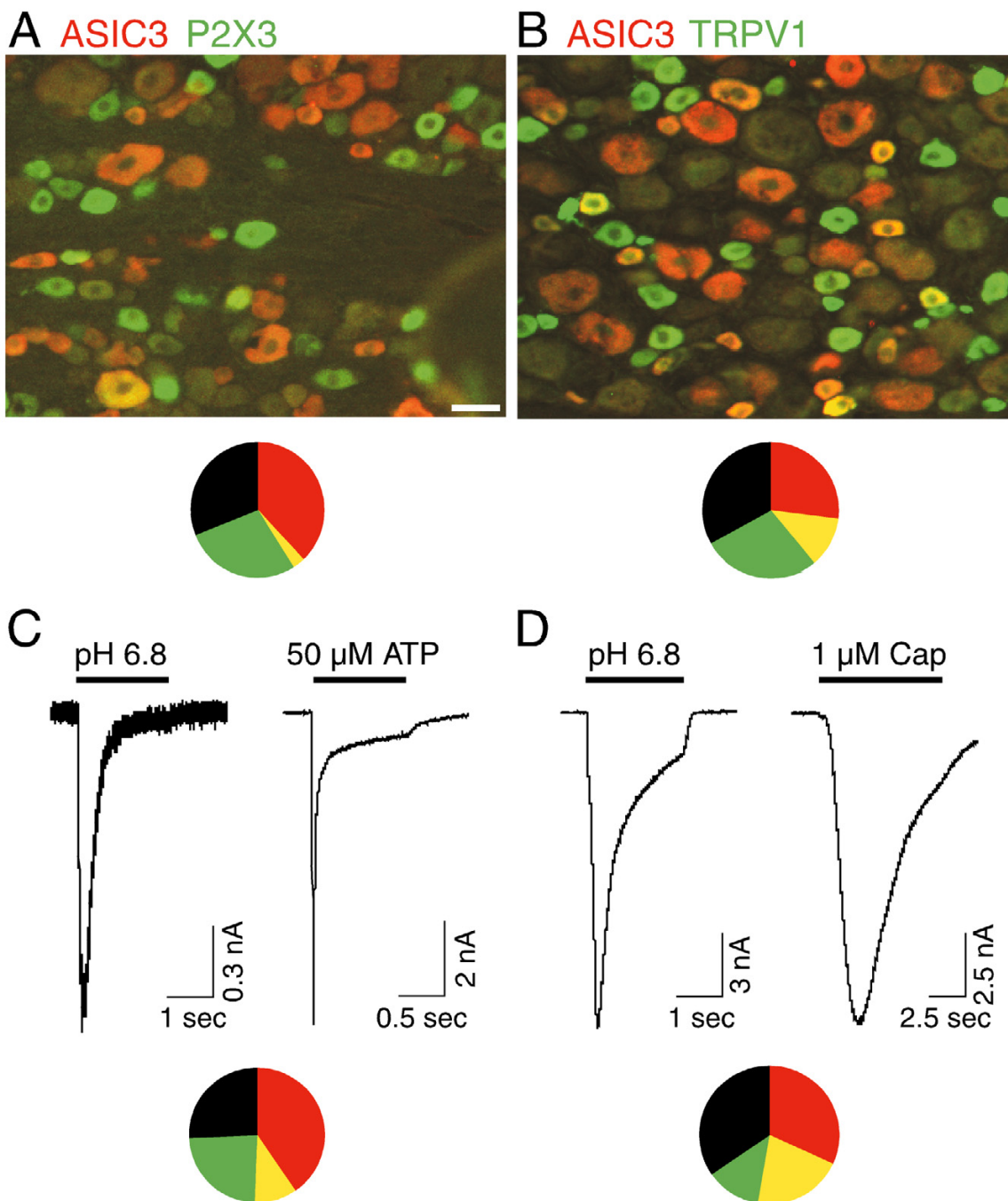
Figure 4 ASIC3 expression compared to other nociceptive ion channels. DRG sections double-labeled for ASIC3 (red) and either P2X3 (green, A) or TRPV1 (green, B); double-labeled cells are yellow or orange. Circle charts show the relative distribution of the three receptors among all DRG neurons. ASIC3 and P2X3 expression overlapped in only 4% of neurons, while some 35% of ASIC3-positive neurons also express TRPV1. The rare cells positive for both ASIC3 and P2X3 were large (eg. cell at lower left in A). 1406 cells counted for A; 995 for B. C, D, electrophysiological recordings reveal a qualitatively similar expression pattern for currents conforming to ASIC3, P2X3, or TRPV1. The cell that generated the currents in C counts as a co-expressor of ASIC3 and P2X3, fitting into the yellow bin in the circle plot. The cell in D is a co-expressor of ASIC3 and TRPV1. Cells were counted positive if they had at least 0.3 nA of current in response to pH 6.8 (ASIC3+), 50 μM ATP (P2X3+; transient current only), or 1 μM capsaicin (TRPV1). 182 cells recorded for C; 169 for D.
