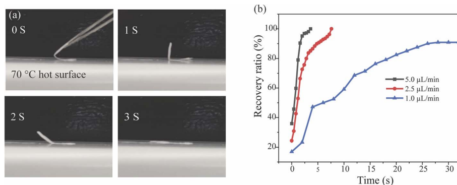
Fig. 6 (a) The digital images of the shape memory effect process of the bended tD /PS (35 wt%) electrospun web using 5 \mu\text{L min}^{-1} flow rate at 70^\circ\text{C} ; (b) the shape recovery ratios as a function of the heating time for electrospun fibers with PS solution concentration of 35 wt% at various flow rates ( 1.0 ; 2.5 and 5.0 \mu\text{L min}^{-1} ).
