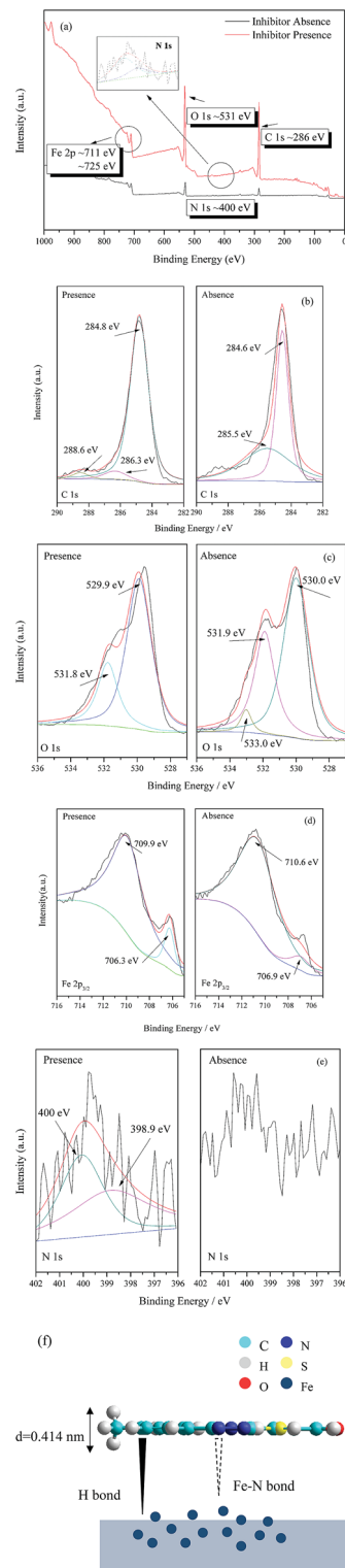
Fig. 5 X-ray photoelectron spectroscopy profiles of (a) full resolution; high resolution (b) C 1s, (c) O 1s, (d) Fe 2p_{3/2} , (e) N 1s for triazole-treated carbon steel and (f) mechanism of inhibitor adsorption.
