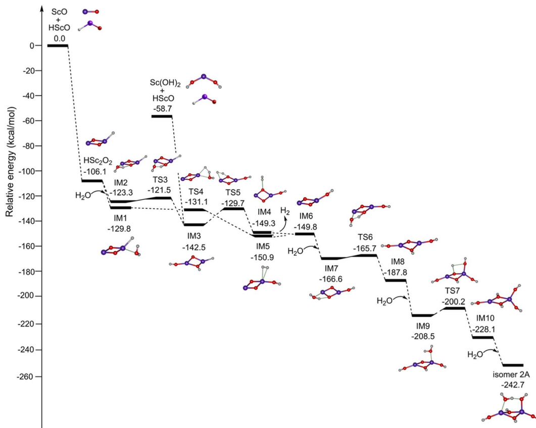
Fig. 4 Potential energy profiles for the formation of \text{Sc}_2\text{O}_6\text{H}_7 (isomer 2A) initiated from the mononuclear non-radical complexes. The abbreviation "IM" stands for intermediate and "TS" for the transition state. Calculations were performed at the TPSSh/def2-TZVP level of theory. Corresponding structures are embedded in the inset (O, red; H, light gray; Sc, purple).
