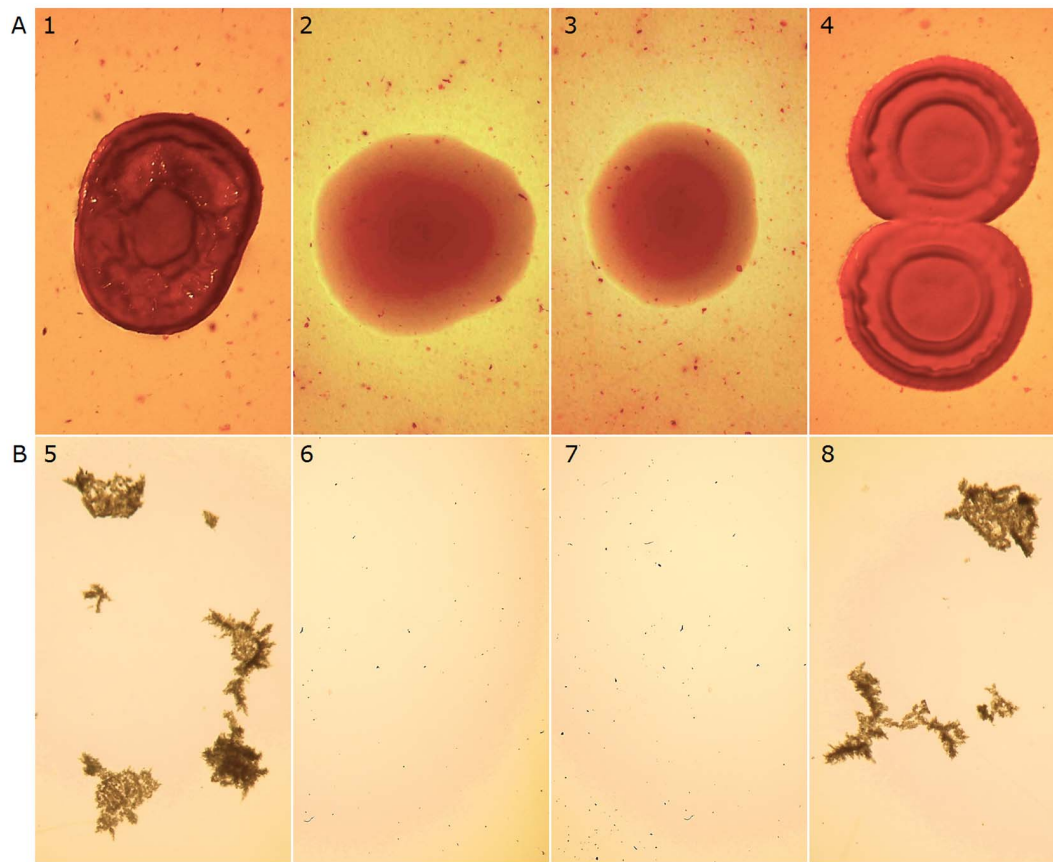
Fig. 1. Congo-red binding and flocculation of A. brasilense strains. A. Wild type strain Sp7 (1) and fliC complemented strain Sp7- fliC Δ[pAB2053] (4) form dark red, rough surfaced colonies on NFM agar containing Congo-Red, whereas, Sp7- fliC Δ (2) and Sp72001 (3) form light-red, mucoid, smooth-surfaced colonies on the same medium. B. Flocculation of Sp7 (5) and Sp7- fliC Δ[pAB2053] (8) in flocculation liquid medium; Sp7- fliC Δ (6) and Sp72001 (7) do not flocculate under the same conditions.
