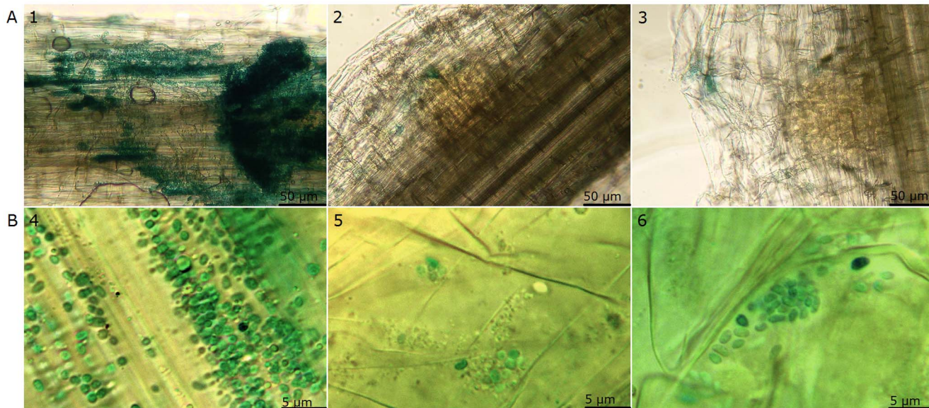
Fig. 2. Plant-root binding abilities of A. brasilense strain. Colonization of wheat root by Sp7 (1 and 4), Sp7- flcA Δ (2 and 5) and Sp72001 (3 and 6). A. brasilense strains harbor the reporter plasmid pLA- lacZ , containing a constitutively expressed lacZ gene and were stained with X-gal. Sp7 (1, 4) has strong binding ability to wheat roots and can be found all over the root surface; Sp7- flcA Δ (2, 5) and Sp72001 (3, 6) lost the ability to bind to wheat roots and could only be found in lateral root emergence areas. Scale bars indicate 50 μm (group A) and 5 μm (group B) (Magnification × 100 in group A and × 1000 in group B).
