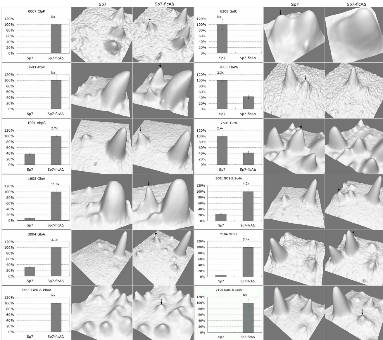
Fig. 4. Differential protein expression in Sp7 and Sp7-fliCΔΔ analyzed by 2-DE. The left section shows the normalized expression volume of the spot in wild type (Sp7) and fliC knock out strain (Sp7-fliCΔΔ) under flocculation conditions; the relative fold change is shown above each column (Nx indicates that relative fold change could not be calculated as the protein was only detected in either Sp7 or Sp7-fliCΔΔ). The right section is a 3D representation of the area of interest as provided by PDquest software. Arrows indicate spots with relatively higher expression.
