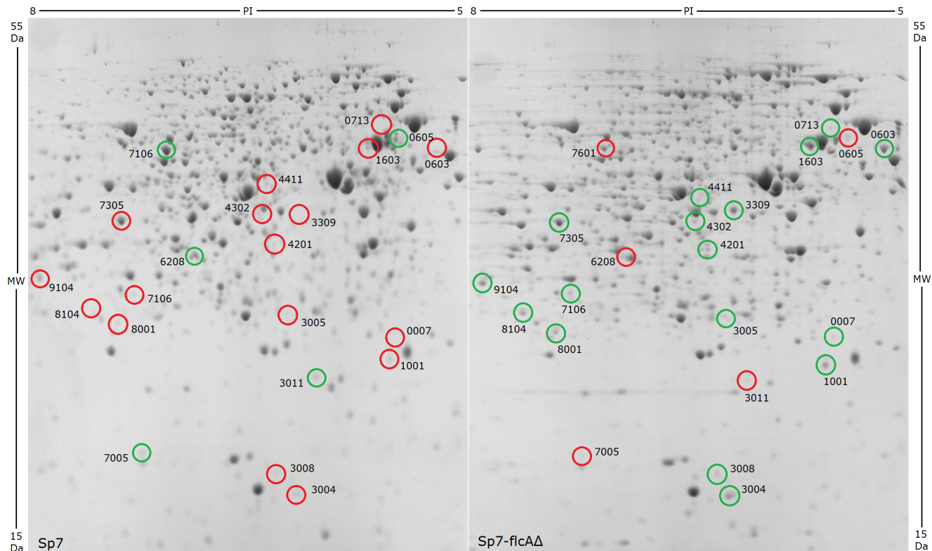
Fig. 3. 2-DE gels of A. brasilense Sp7 and Sp7- fliC Δ under flocculation conditions. Blue silver stained 2-DE gel of proteins extracted from Azospirillum Sp7 (A) and Sp7- fliC Δ mutant (B) under flocculation conditions. Circled spots were found to be differentially expressed and were able to be excised and analyzed by LC-MS/MS. Green circles indicate increased expression and red circles indicate decreased expression in either Sp7 or Sp7- fliC Δ.
