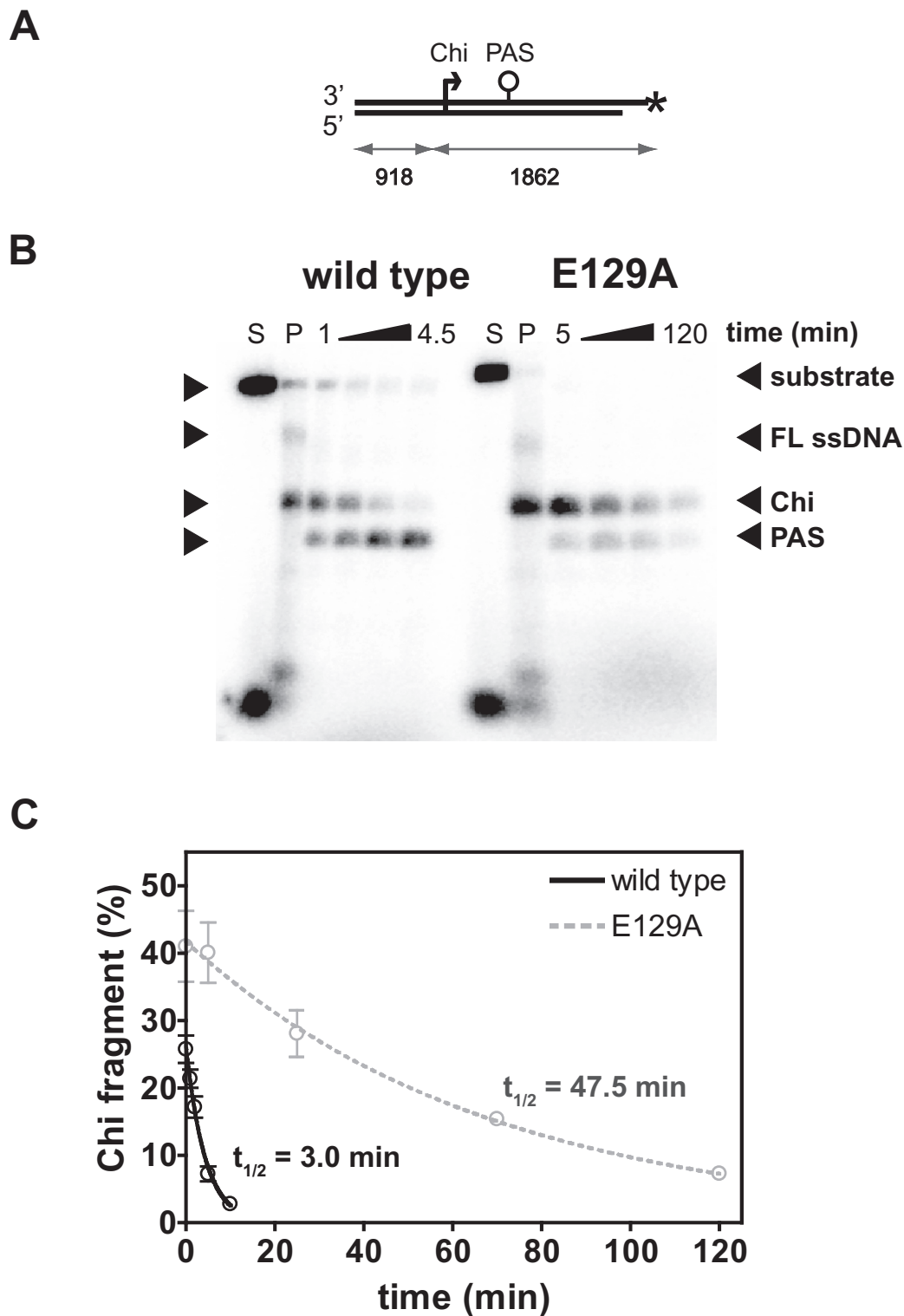
Figure 3. Disruption of the ionic latch results in the formation of hyper-stable AddAB-Chi complexes. (A) Schematic of the DNA substrate used in these experiments. AddAB can only enter from the left of these substrates as shown. The positions of a single Chi sequence and primosome assembly site (PAS) are highlighted. The asterisk marks the position of a radiolabel. (B) Exonuclease chase assay to measure stability of the AddAB:Chi complex. Lane S shows unprocessed substrate DNA, and lane P shows the products of AddAB resection assays, which is used to estimate the initial yield of Chi fragment. Subsequent time points (indicated) are from the Exonuclease chase reaction start time. 1.6 nM DNA molecules were processed by 4 nM AddAB enzymes in the presence of 2 \mu M SSB and 1 mM ATP at 37°C. ExoI was added to a final concentration of 0.8 units/ \mu l. Black triangles mark the DNA substrate, full length (FL) ssDNA, the Chi fragment and the primosome assembly site (PAS; a region of secondary structure that is ExoI resistant (8)). Gels have been uniformly contrast enhanced to aid visualisation of reaction products. (C) Quantification of total Chi fragment as a function of time. Both data sets were fit to a single exponential decay to zero. The half life ( t_{1/2} ) is indicated. Error bars represent the SEM derived from three independent experiments.
