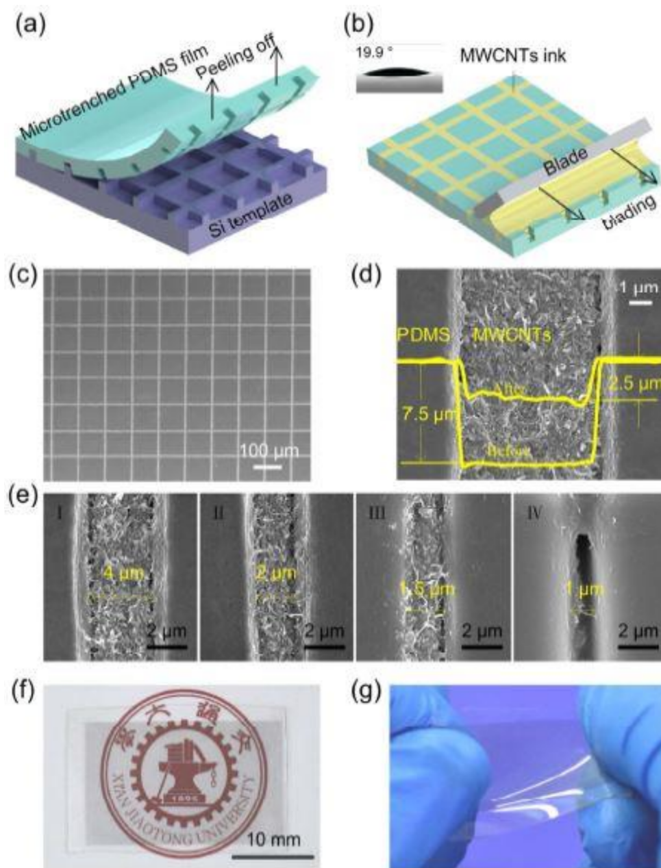
Figure 2. (a,b) Fabrication process of the multi-walled carbon nanotube (MWCNT)-based sensors formed using flexible PDMS films having mesh-like microtrenches. (c) Scanning electron microscope (SEM) images of the developed sensors with MWCNTs embedded in the microtrenches. (d) Profiling of the microtrenches before and after the embedding process. The formed sensors were kept in (e) normal, (f) weisting positions and (g) Representation of high stretchability of the sensors. [74]. Reproduced from Nie, B.; Li, X.; Shao, J.; Li, X.; Tian, H.; Wang, D.; Zhang, Q.; Lu, B. Flexible and transparent strain sensors with embedded multiwalled carbon nanotubes meshes. ACS Appl. Mater. Interfaces 2017 , 9 , 40681–40689.
