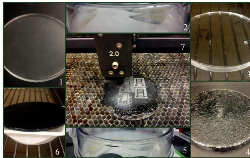
Figure 4. Representation of the steps of fabrication that were followed to develop the MWCNT/PDMS-based strain sensors [107]. Reproduced from Nag, A.; Mukhopadhyay, S.C.; Kosel, J. Flexible carbon nanotube nanocomposite sensor for multiple physiological parameter monitoring. Sens. Actuators A Phys. 2016 , 251 , 148–155.
