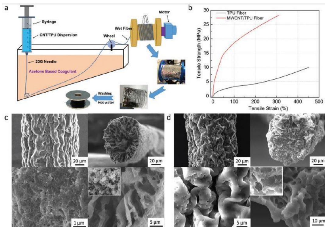
Figure 5. (a) Schematic diagram of the wet spinning process of the MWCNT-based composites. (b) Stress–strain curve of the composites. (c,d) SEM images of the composite fibers [91]. Reproduced from He, Z.; Zhou, G.; Byun, J.H.; Lee, S.K.; Um, M.K.; Park, B.; Kim, T.; Lee, S.B.; Chou, T.W. Highly stretchable multi-walled carbon nanotube/thermoplastic polyurethane composite fibers for ultrasensitive, wearable strain sensors. Nanoscale 2019, 11, 5884–5890.
