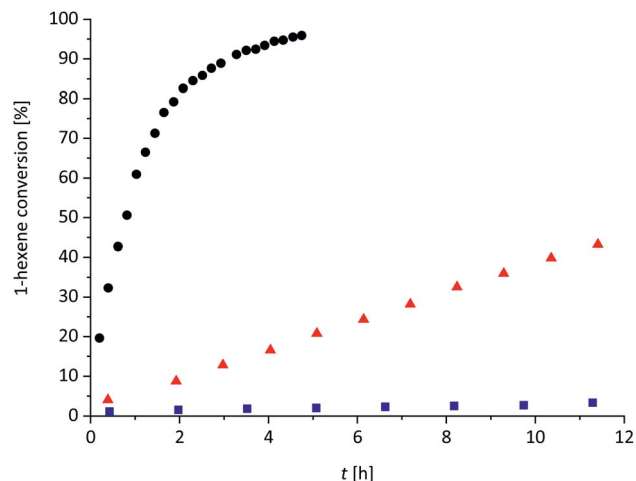
Fig. 1 Plot of 1-hexene conversion versus time for the catalytic hydrosilylation reaction of 1-hexene with 1.2 eq. \text{Me}_3\text{SiH} and 10 mol% 1 (black dots), with 1.2 eq. \text{Me}_3\text{SiH} and 1 mol% 1 (red triangles) and with 1.0 eq. \text{Me}_3\text{SiH} and 0.5 mol% 1 (blue squares) in o DFB (0.11 M for 1-hexene) at rt. The 1-hexene conversion was obtained by ^1\text{H} NMR integration (1-hexene conversion = c(\text{RH}_2\text{C}-\text{H}_2\text{C}-\text{SiMe}_3)/c(\text{RH}_2\text{C}-\text{H}_2\text{C}-\text{SiMe}_3 + \text{H}_2\text{C}=\text{CH}-\text{R}) ; \text{R} = \text{nBu} ).
