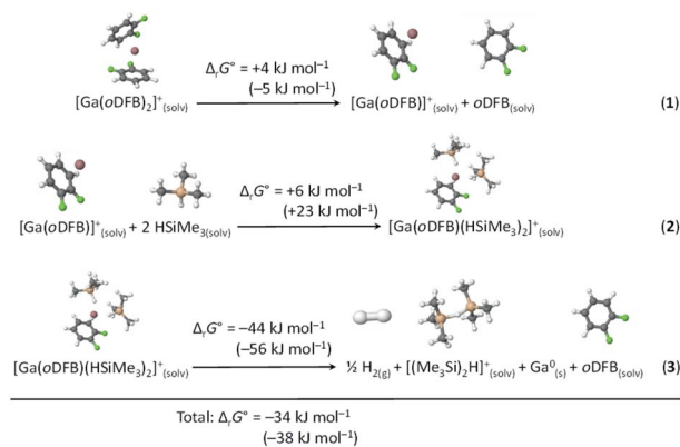
Scheme 4 Calculated Gibbs free energies \Delta_r G^\circ ( oDFB solution, calculated with the COSMO model, \epsilon_r = 13.38 66 ) for the dissociation of [Ga(oDFB)_2]^+ (reaction (1)), subsequent addition of two HSiMe_3 molecules to yield [Ga(oDFB)(HSiMe_3)_2]^+ (reaction (2)), and its decomposition to give H_2 , Ga^0 , oDFB and [(Me_3Si)_2H]^+ (reaction (3)). The Gibbs free energies were calculated at the RI-BP86(D3BJ)/def2-TZVPP level at 298 K (values in parentheses: RI-B3LYP(D3BJ)/def2-TZVPP). The optimized structures of the involved species are included.
