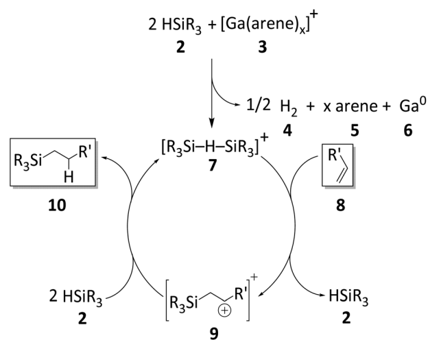
Scheme 5 Proposed catalytic cycle for the hydrosilylation of olefins initiated by Ga^+ (arene = oDFB or PhF). The olefin 8 and the hydrosilylation product 10 are highlighted.
