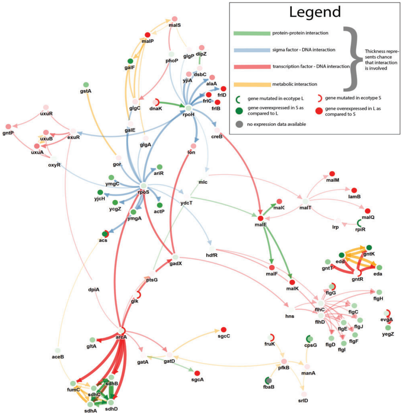
FIG. 4. —Visualization of subnetworks inferred from the coexisting ecotypes data set. The visualization was created by merging separately inferred subnetworks resulting from a parameter sweep of the edge cost from 0.025 to 0.975. The width of the edges represents the maximal 30 mutation cost for which these edges were selected. The width of the edge displays the stringency at which the edge was selected (the wider the edge the more stringent the condition. More stringent conditions correspond to higher edge costs). Node borders are subdivided into two parts to visualize in which strain a mutation occurred. The inner color of the nodes represents the degree of differential expression (L ecotype compared with S ecotype). The colors of the edges represent the edge types.
