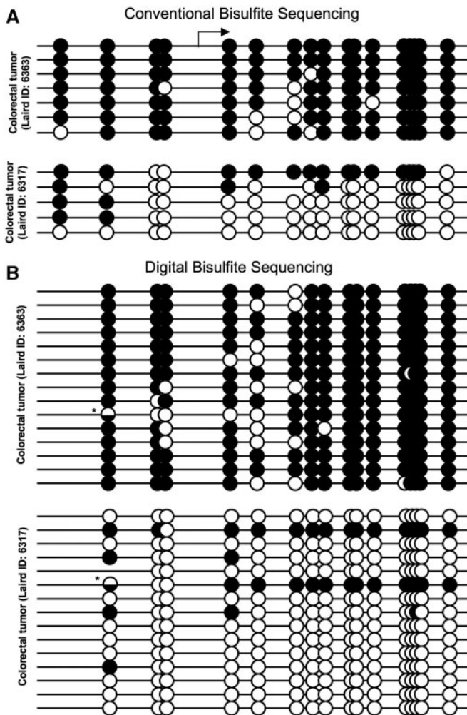
Figure 2. Comparison between conventional and digital bisulfite genomic DNA sequencing of MLH1 CpG island. Bisulfite-converted tumor DNA from two colorectal cancer patients was amplified at the MLH1 locus and subject to (A) TOPO-TA cloning followed by DNA sequencing, and (B) Digital bisulfite genomic DNA sequencing. Each horizontal line represents an individual DNA molecule, and the circles represent CpG dinucleotides. Filled in circles are methylated CpGs while open circles are unmethylated CpGs. The asterisk (*) represents DNA sequencing reads that gave signals for both methylation and the absence of methylation for a specific CpG dinucleotide, and may be indicative of two DNA molecules amplified in the PCR reaction well.
