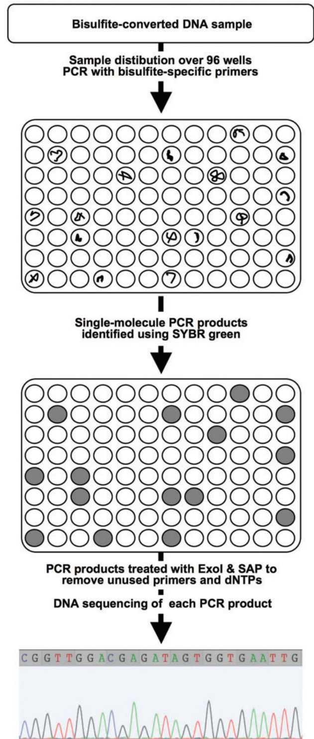
Figure 1. Digital bisulfite genomic DNA sequencing overview. An amount of bisulfite-converted DNA was loaded such that individual template DNA molecules were amplified on a 96-well PCR plate. We targeted a maximum of 20–30 molecules to be sequenced in each PCR plate in order to minimize the occurrence of two or more PCR template molecules per reaction well. Positive amplifications are evaluated by SYBR green melting curve analyses, and PCR products from these wells are removed and purified with Exonuclease I and Shrimp Alkaline Phosphatase (Exo-SAP-IT) to remove unused PCR primers and dNTPs. PCR products representing individual DNA molecules are then subject to DNA sequencing.
