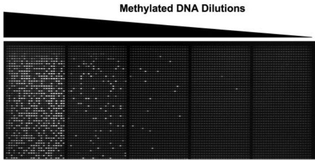
Figure 4. Detection of single methylated PITX2 molecules serial dilutions of bisulfite-converted M.SssI -DNA using microfluidic digital MethyLight (Fluidigm). Each DNA sample was compartmentalized into 1104 reaction chambers of 10 nL each and amplifications were visualized by fluorescence emission in each positive chamber.
