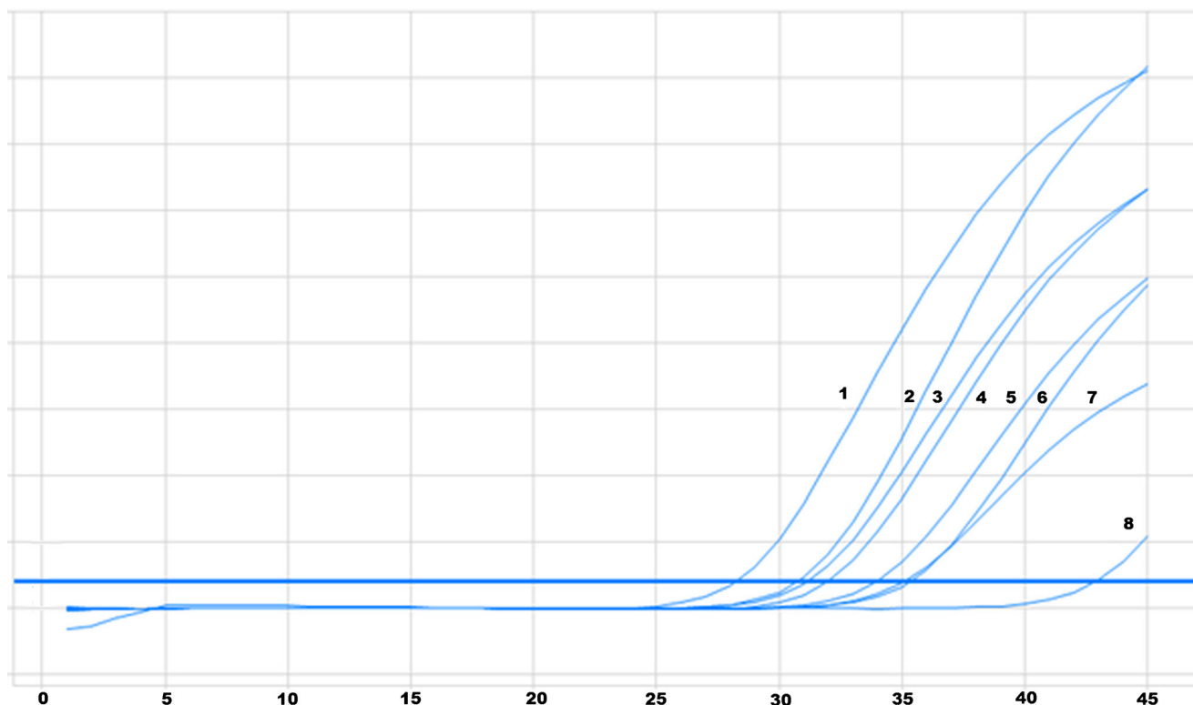
Fig. 1 Amplification curves for DNA with T790M mutation diluted with control DNA and control DNA alone: 1–50 %, 2–25 %, 3–20 %, 4–10 %, 5–5 %, 6–2 %, 7–1 %, 8—control DNA
