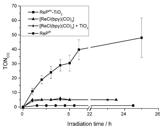
Figure 3. Photocatalytic CO production from CO 2 under \lambda > 420 nm irradiation with the ReP pic -TiO 2 hybrid system compared to homogeneous [ReCl(bpy)(CO) 3 ] with and without TiO 2 and ReP Br in solution (ReP pic is insoluble in DMF). 0.1 \mu mol Re catalyst in 4.5 mL DMF/TEOA 5:1 was used with 5 mg TiO 2 . TON CO = mol CO mol Re -1 .
