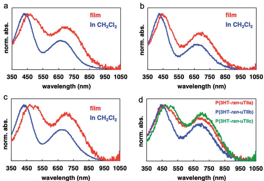
Fig. 2 UV-vis absorption spectra of (a) P(3HT- ran -uTIIa), (b) P(3HT- ran -uTIIb), (c) P(3HT- ran -uTIIc) in film and solution states, and (d) all three polymers in the film state.
